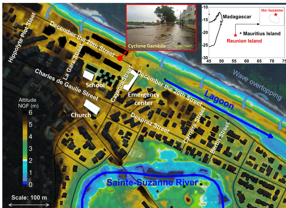
Figure 1: Topography of Sainte-Suzanne city derived from high-resolution LIDAR (IGN) data with main streets and critical buildings of the sea-front quarter.
