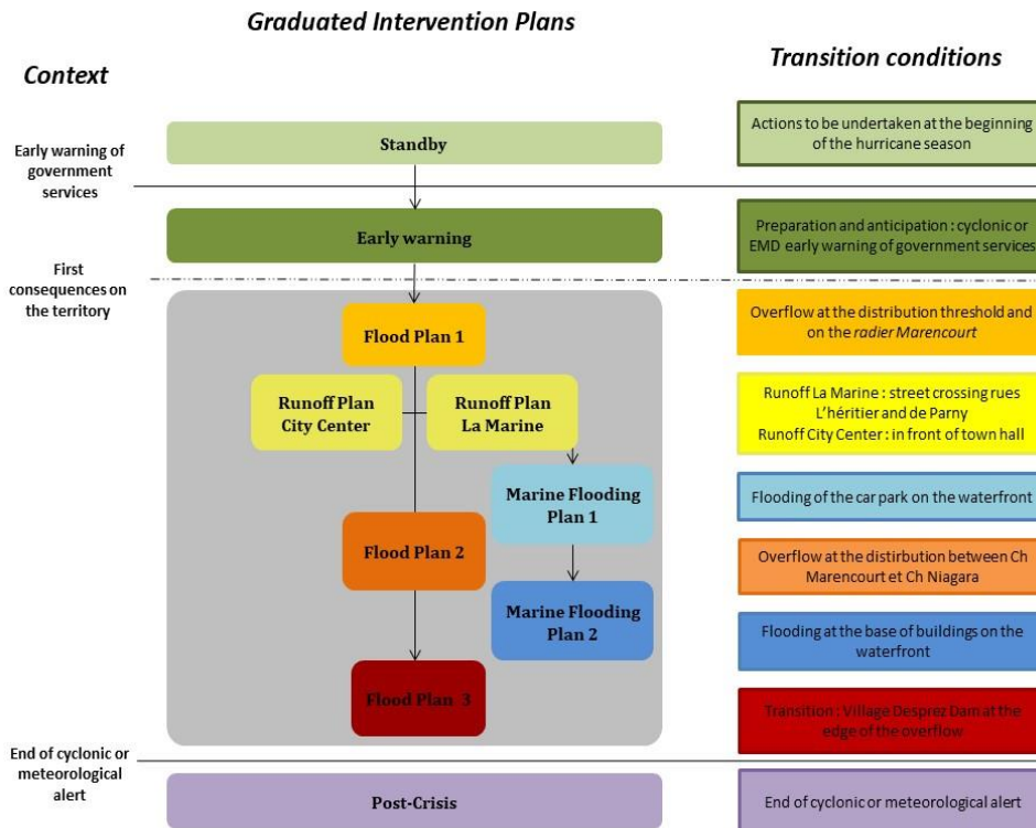
Figure 7. Complete GIP for a cyclonic event including runoff, marine flooding and river flooding.
