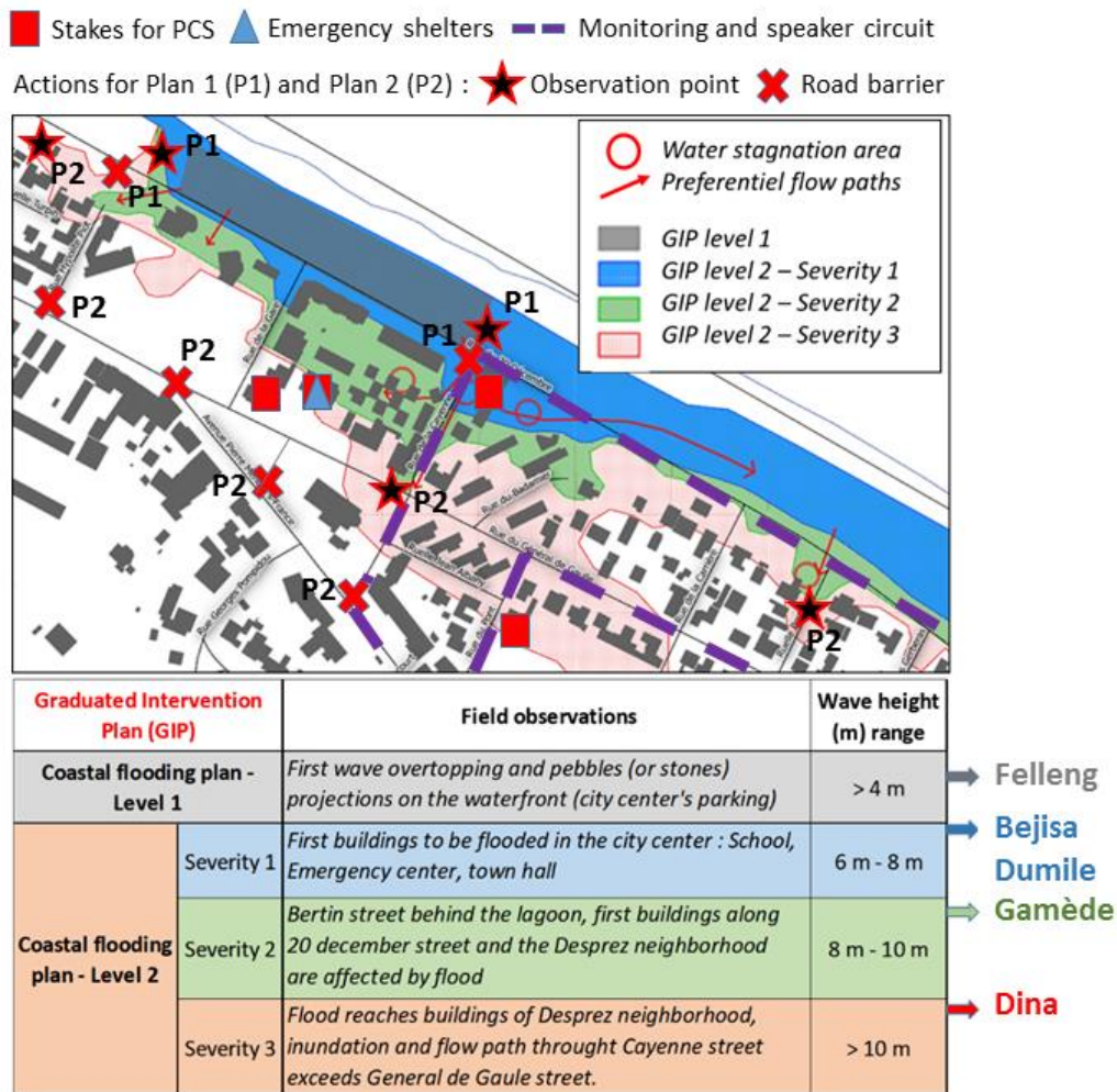
Figure 6: Map aggregating the different levels of the Graduated Intervention Plan (GIP) of Sainte Suzanne city centre with the transition criteria (field observations, Hs thresholds and benchmarks).
