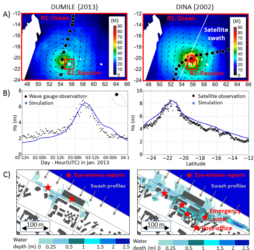
Figure 2: A) Grid extent with tracks (black dots), wind intensity (colors) and directions (arrows) of cyclones Dina and Dumile calculated with MESO-NH from best-track data. B) Comparison between simulated wave heights with observations from satellite altimetry on January the 23 rd at 06 UTC (Dina) or time-varying observations from buoy RN4 (Dumile). C) Position of the SWASH profiles and comparison between simulated flooding with eyewitness accounts.
