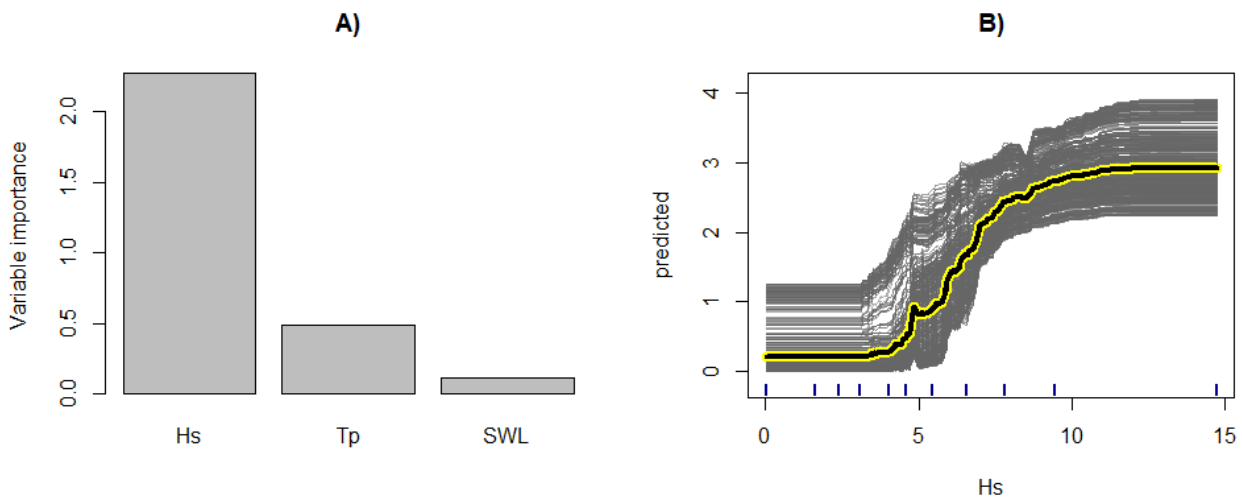
Figure 4: A) Importance measure for each variable ( H_s , T_p , SWL ) derived from a random-forest model trained using the synthetic cyclones B) Functional relationship between the predicted value of the log-transformed of V and H_s . The yellow line indicates the average effect of H_s .
