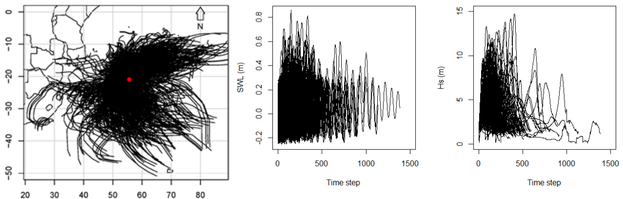
Figure 3: 500 synthetic tracks constituting the database with examples of 30 time series (presented on a normalized time index) of significant wave heights (Hs) and seawater levels (SWL) at 50m depth in front of Sainte-Suzanne city.
