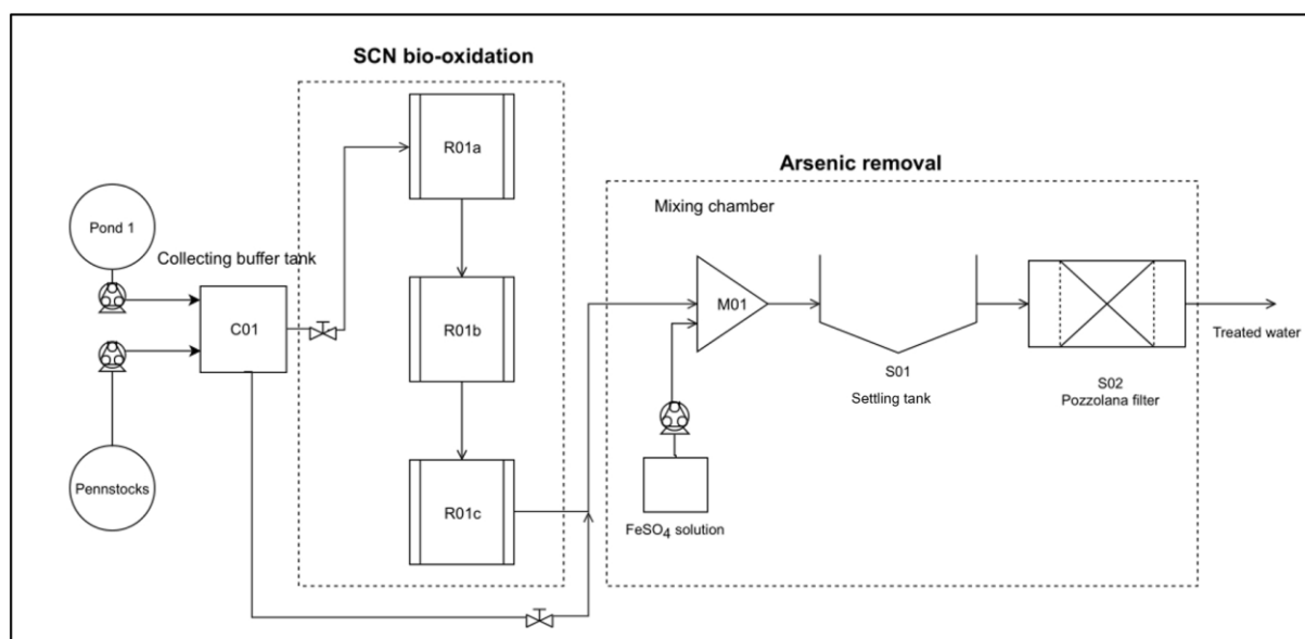
Figure 5 Process flow diagram of on-site pilot experiment.
