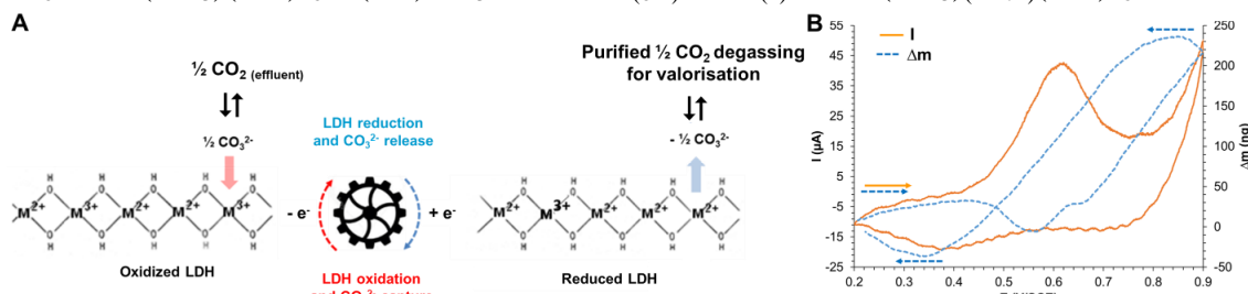
Fig. 1: A. Electrolytically supported processes of capture and release of CO 3 2- using LDHs. B: Coupling of CV and QCM, using thin LDHs films, coated on platinum-based quartz electrodes.
