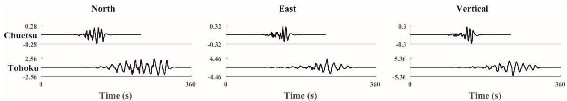
Figure 4. North, East and vertical components of displacement histories in cm at station GIF023 corresponding to events listed in Table 1.
