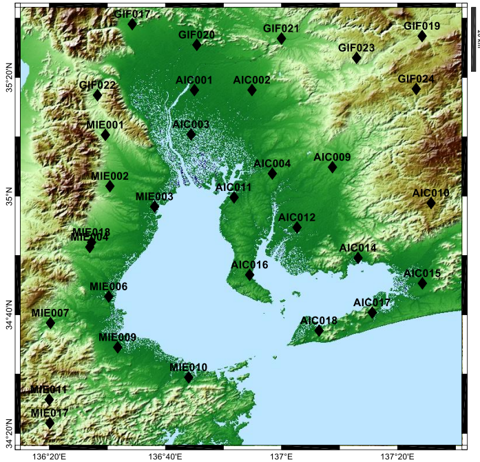
Figure 2. Location of K-net seismic stations used in the study.
