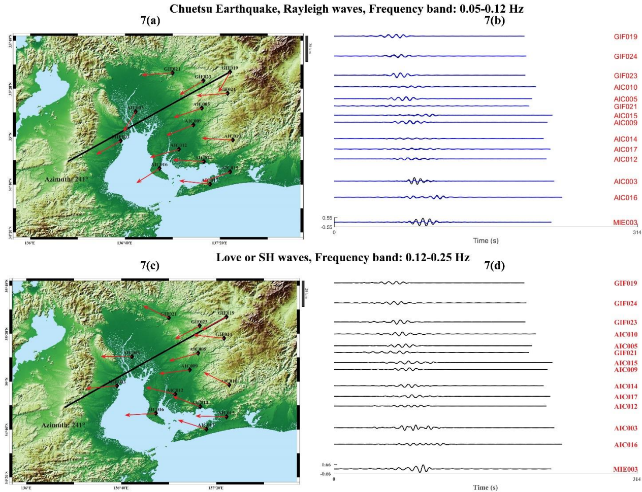
Figure 7. Surface waves extracted from recording of Chuetsu Earthquake. The red arrows indicate the direction of polarization.
