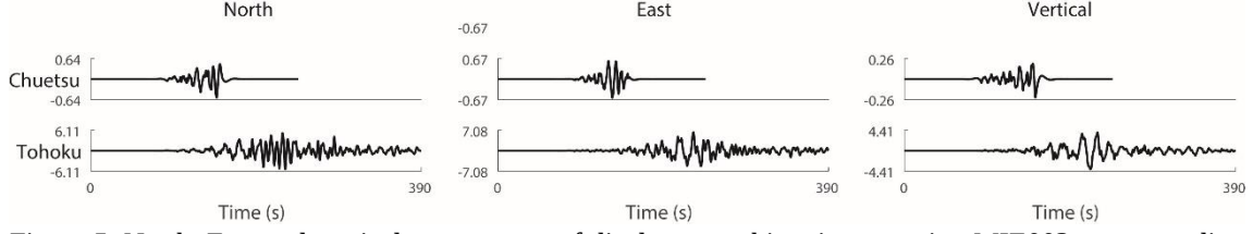
Figure 5. North, East and vertical components of displacement histories at station MIE003 corresponding to events listed in Table 1.
