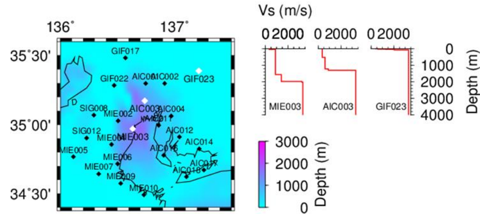
Figure 3. The upper depth of a layer of V_s=2700 m/s from the 3D deep structure model provided by NIED. The V_s profiles are also shown for the three stations MIE003, AIC003 and GIF023.
