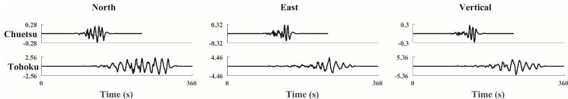
Figure 4. North, East and vertical components of displacement histories in cm at station GIF023 corresponding to events listed in Table 1.
