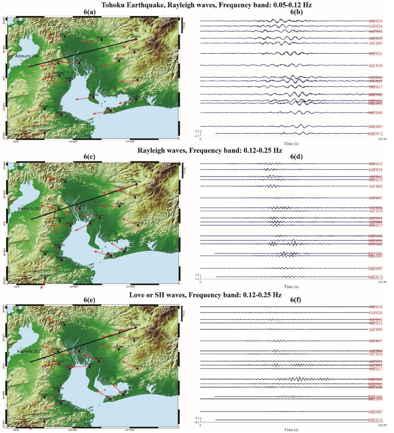
Figure 6. Surface waves extracted from recording of Tohoku Earthquake. The red arrows indicate the direction of polarization.
