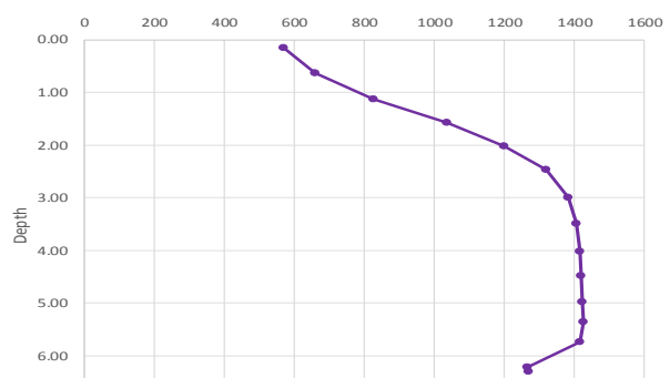
Fig. 2: Conductivity profile by multiparametric probe ( \mu S/cm) in shallow groundwater, BH19.
