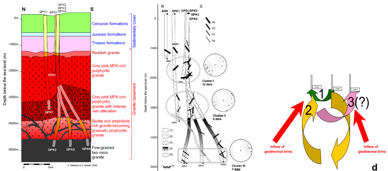
Figure: Geological conceptual model of the Soultz granite (left). Fracture zones cross-cut in the wells (center). Conceptual model of fluid circulation in the Soultz geothermal reservoir (Sanjuan et al. , 2006) (right).
