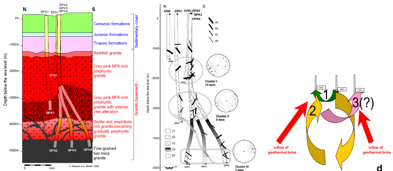
Figure: Geological conceptual model of the Soultz granite (left). Fracture zones cross-cut in the wells (center). Conceptual model of fluid circulation in the Soultz geothermal reservoir (Sanjuan et al. , 2006) (right).
