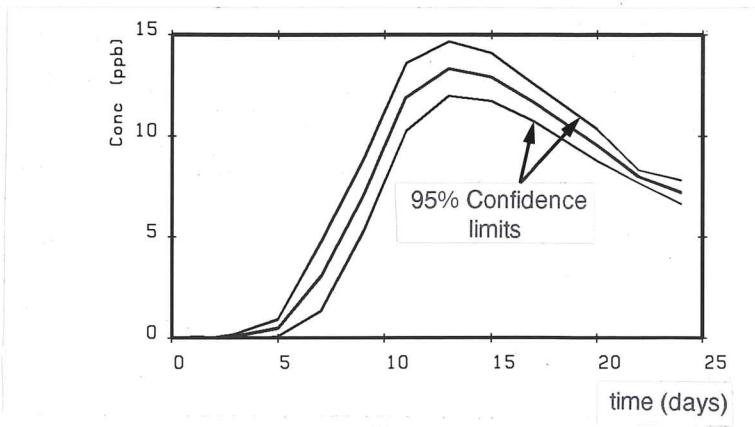
Fig. 7 - Finnsjon tracer test : concentration prediction corresponding to other injection and pumping rates.
