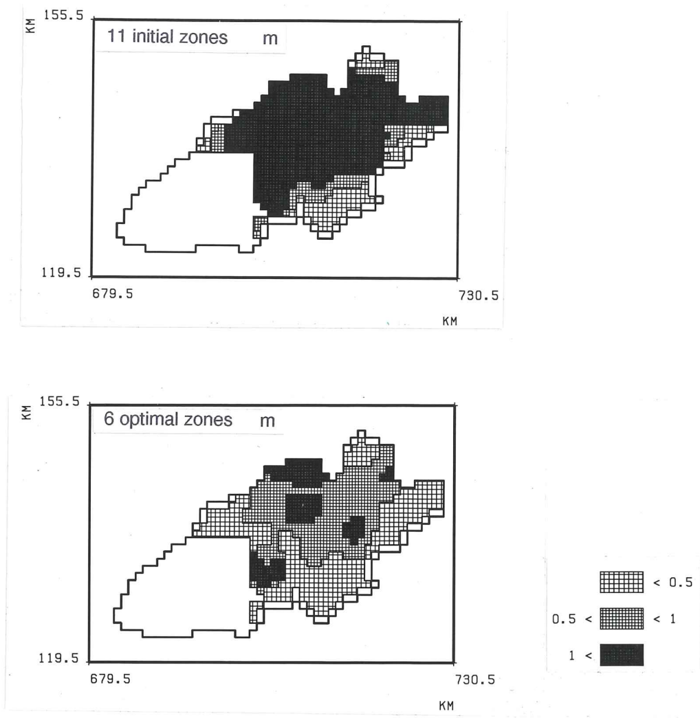
Fig. 6 - Thau aquifer : standard deviation of hydraulic heads simulation.
