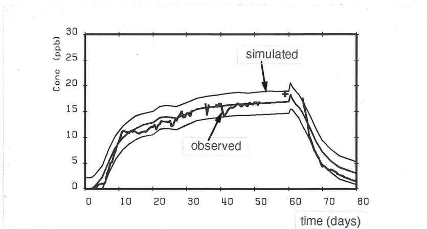
Fig. 4 - Finnsjon tracer test : comparison of simulated and observed concentrations with 95 % confidence limits.
