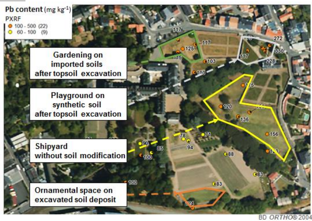
Fig. 6: Example of multiple contaminated soil management options, including NBS for Eglantiers (a) and Oblates (b) UAGs
