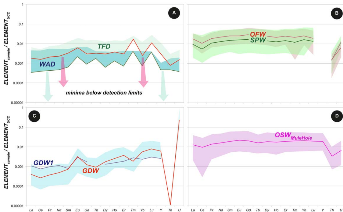
Figure 4. UCC-normalized REY-Th-U patterns for (a) wet atmospheric and throughfall deposits, (b) soil inputs (overland flow water) and soil outputs (soil pore waters), (c) stream water, and (d) groundwater. The shadow regions represent the variability.
