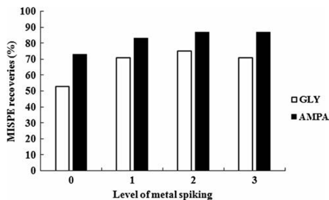
Fig. 2 Elution recoveries ( n = 1 ) of GLY and AMPA in groundwater spiked at four levels of metal concentration (Table 1). Experimental conditions described in the “Determination of metal interferences in real matrices” section
