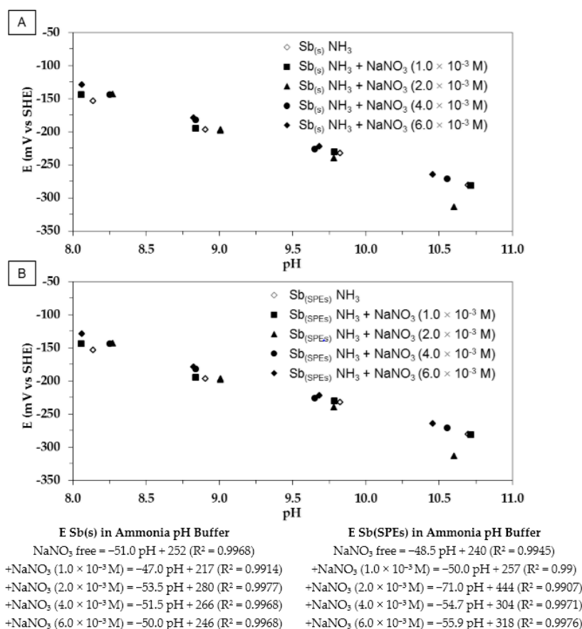
Figure 5. Eh-pH diagram of both Sb(s) (A) and Sb(SPEs) (B). Experiments were done at 25 °C, at atmospheric pressure, in ammonia pH buffer solutions ( I_S = 0.1 ) containing \text{NaNO}_3 ( 0 , 1.0 \times 10^{-3} , 2.0 \times 10^{-3} , 4.0 \times 10^{-3} and 6.0 \times 10^{-3} M).
