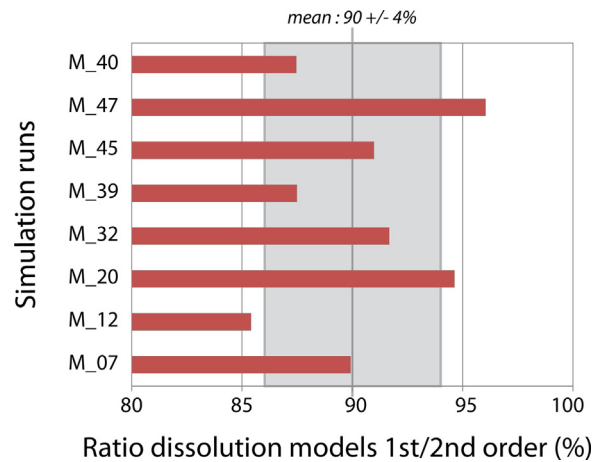
Fig. 5. (Color online.) Ratio between models with and without second-order heterogeneity of dissolved CO 2 for each simulation after 50 years of injection.
