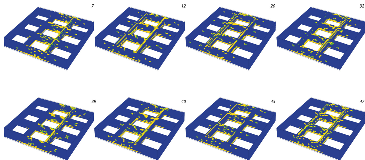
Fig. 2. (Color online.) Representation of eight second-order heterogeneity models selected for the flow simulations with TOUGH2-MP. The connectivity of the reservoir bodies sharply differs from one model to another and it results from the stochastic pattern of the algorithm (Issautier et al., 2014).
