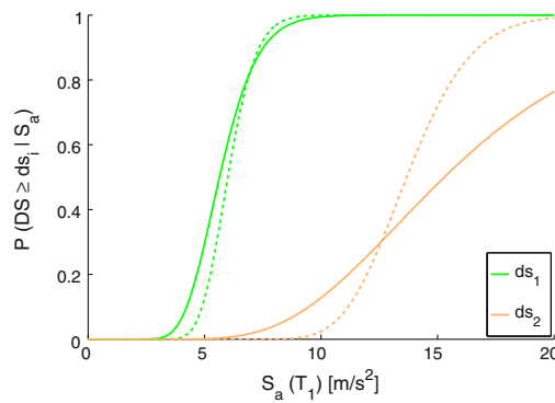
Fig. 5. Fragility functions derived by FRACAS using the GLM (solid lines) and the LS fitting (dashed lines) for the Special-Code building, TRI-PO, and EPP model.
