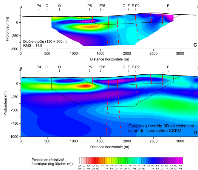
Figure 3 Cross section extracted from the 3D resistivity model and 2D long DC resistivity profile.
