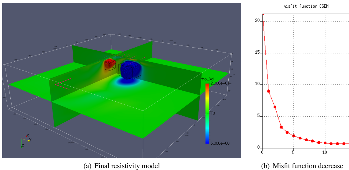
Figure 1 3D resistivity model obtained by frequency-domain CSEM data inversion, using 121 stations, 2 source polarisations and 6 frequencies from 0.5 to 128Hz.
