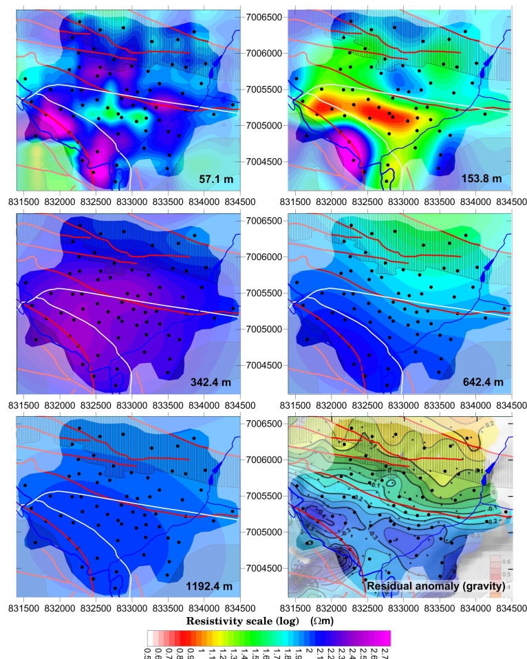
Figure 2 Slices of the 3D resistivity model and (f) gravity map, with contours from the geological map.
