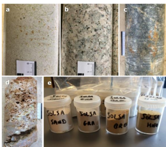
Figure 1. Sonic drilled cores (Royal Eijkelkamp, NL) of sandstone (a), and granite (b); diamond drilled cores (SLN, NC) of serpentinized harzburgite (c) and breccia (d); e: powdered samples (< 80 \mu\text{m} ) of the abovementioned sample materials.
