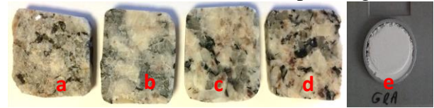
Figure 4: Granite samples – a: as-drilled; b: as-sawn; c: polished at 6 \mu\text{m} ; d: polished at 0.25 \mu\text{m} ; e: crushed to powder.
