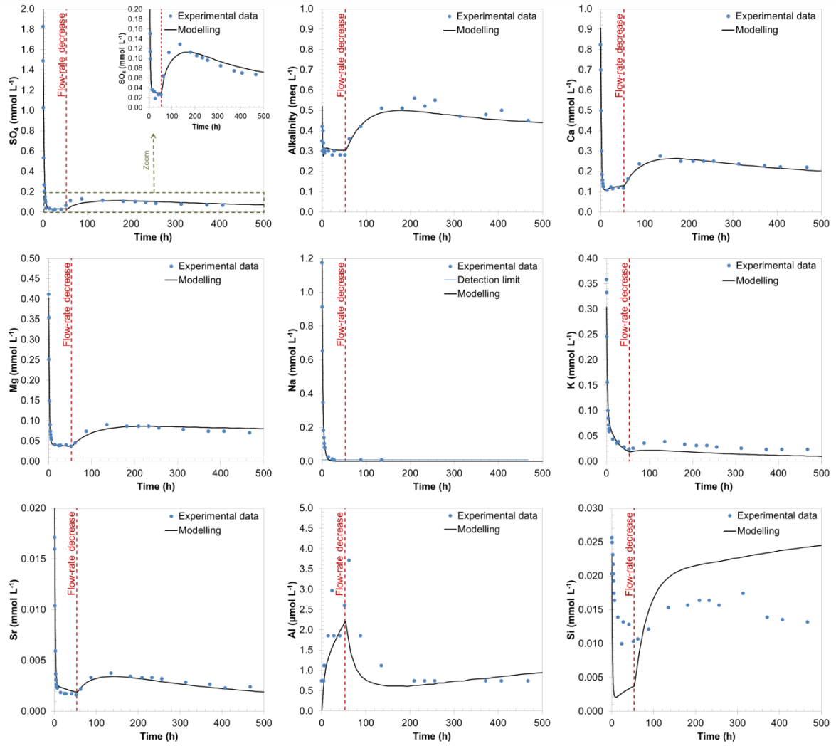
Fig. 1. Evolution of outlet solution composition as function of time (alkalinity as well as \text{SO}_4 , Ca, Mg, Na, K, Sr, Al and Si concentrations).
