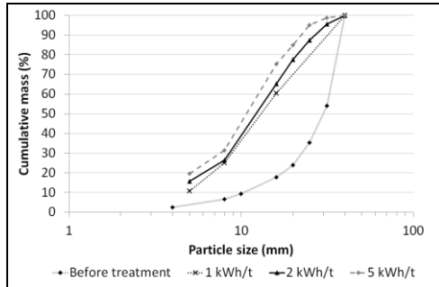
Figure 3. Particle size distribution of the fragments obtained at various discharged energy.
