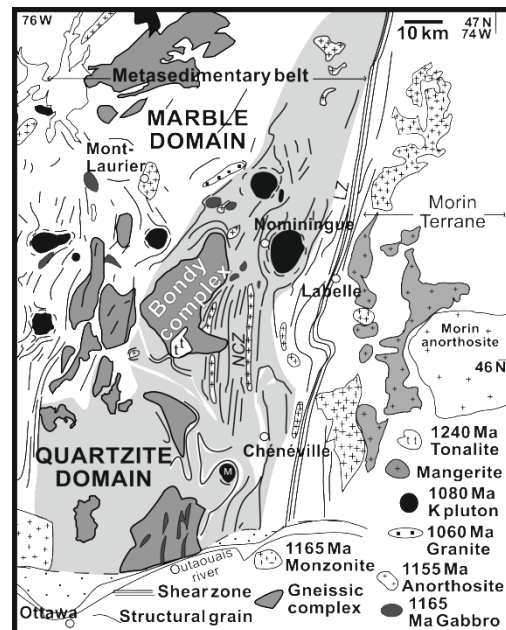
Figure 1. Location of the Bondy complex within the Central Metasedimentary Belt of the southwestern Grenville Province in Québec (modified from Corriveau and van Breemen 2000).
