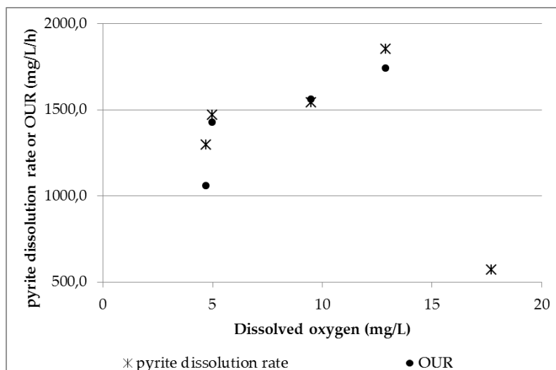
Figure1: Pyrite dissolution rate and OUR vs. DO concentration in continuous pyrite bioleaching experiments
