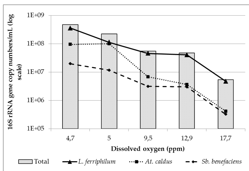
Figure 2: Influence of DO concentration on the microbial community structure and the quantity of biomass present in the reactor (assessed using the number of 16S rRNA gene copy)
