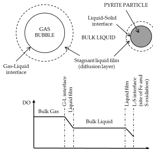
Figure 4: Schematic description of oxygen transfer and oxygen concentration profile in a triphasic media with reactions consuming oxygen at the solid surface
