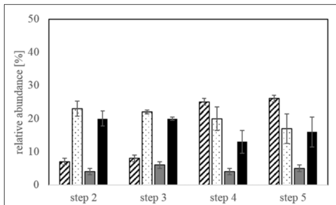
FIGURE 4 | Relative abundance of the four different species ( Leptospirillum ferriphilum -hatched bars, Acidithiobacillus caldus -dotted bars, Sulfo bacillus benefaciens -gray bars, Sulfo bacillus thermosulfidooxidans -black bars) in the bioleaching reactors at the end of each bioleaching experiment determined by qPCR. Data are mean values of triplicates \pm SD.
