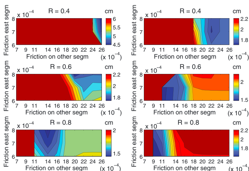
Figure 6. Variation of the WRMS misfit for the GPS data set. (left column) The result for an orientation of 50^\circ and (right column) the result for an orientation of 60^\circ . The y axis is the b friction constant on the eastern Léogâne segment, and the x axis is the b friction constant on the other segments where b is the constant from equation (4).
