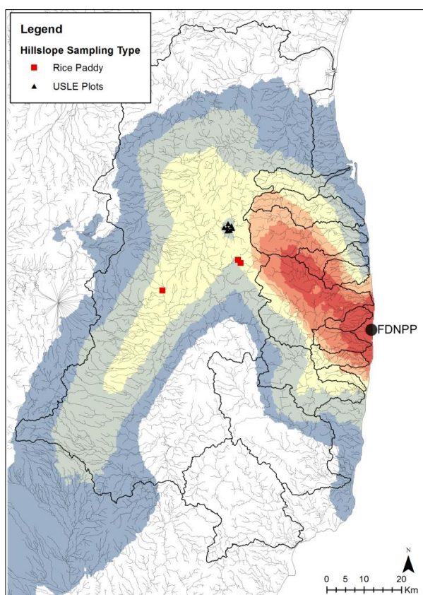
Figure 7. Sample locations for research examining hillslope radiocesium transfer with USLE-based and calculations of suspended sediment yields form rice paddy fields.
