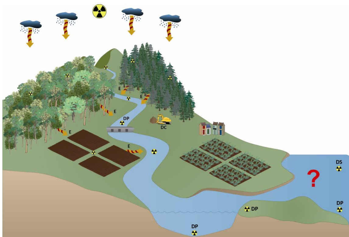
Figure 2. Potential pathways for radiocesium transfer from hillslopes to the Pacific Ocean following the FDNPP accident denoting major processes such as erosion (E), deposition (DP), decontamination (DC) and desorption (DS) (Images courtesy of the Integration and Application Network, University of Maryland Center for Environmental Science ( ian.umces.edu/symbols/ )).
