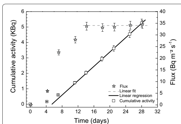
Fig. 10 Example of a typical diffusion curve (squares) and flux curve (stars), with the linear regression of the steady state part of the diffusion curve (full line) and of the flux curve (dashed line). The linear regression (solid line) represents the fit of the steady state part of the cumulative activity curve (constant flux, dashed line). The intercept a and the slope b of the linear regression gives the porosity \varepsilon_a and effective diffusivity D_e , respectively (see Eqs. 2, 3).
