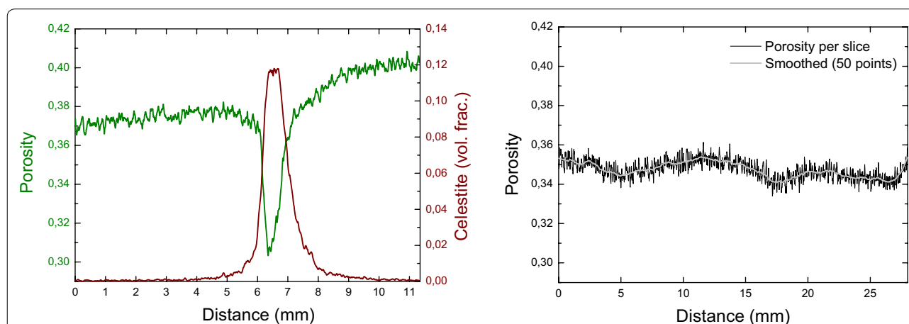
Fig. 5 Precipitated celestite and porosity profile in diffusion cell Prec1 (left) and in a reference diffusion cell without celestite precipitation (right) using voxel-counting.
