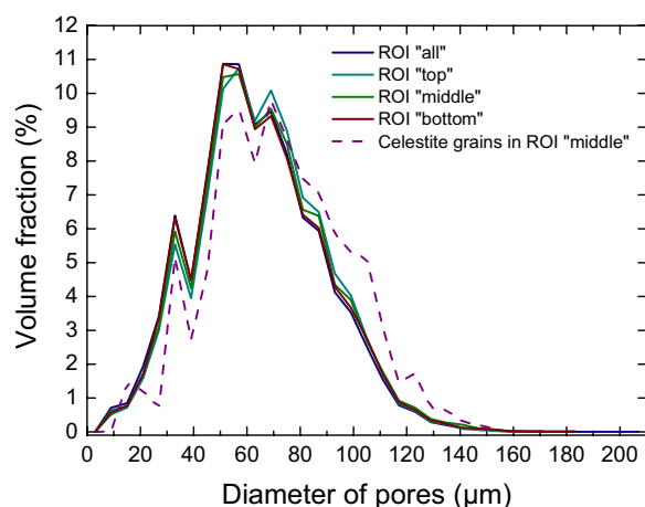
Fig. 8 Geometric pore size distribution and celestite grain size distribution calculated with the pore morphology model for different ROIs.
