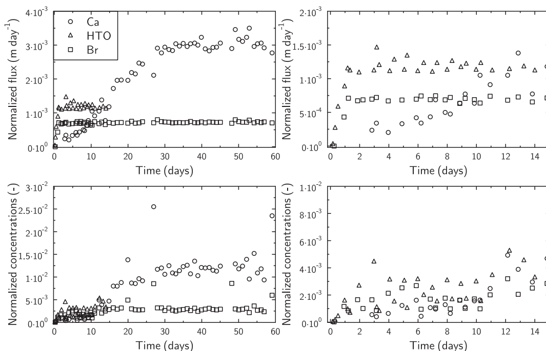
Fig. 3. Top: Comparison of normalized mass flux densities as a function of time for Ca (circles), HTO (triangles), and Br (squares). Bottom: Comparison of normalized concentrations (same symbols). Right figures show the results for the first 15 days of the diffusion experiments.
