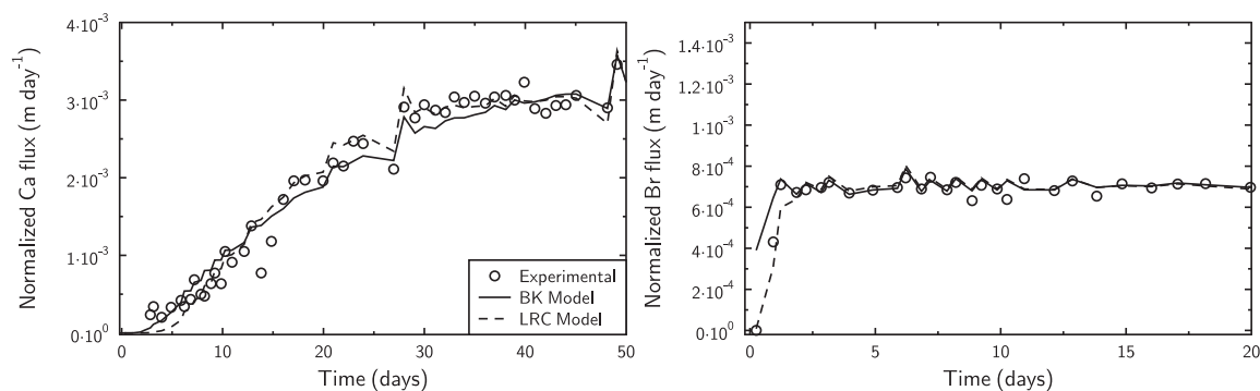
Fig. 11. Ca (left) and Br (right) mass flux densities as a function of time: experimental data (open circles), BK model (full lines), and LRC model (dashed lines). See Fig. 1 for a description of models, and Table 3 for model parameters.
