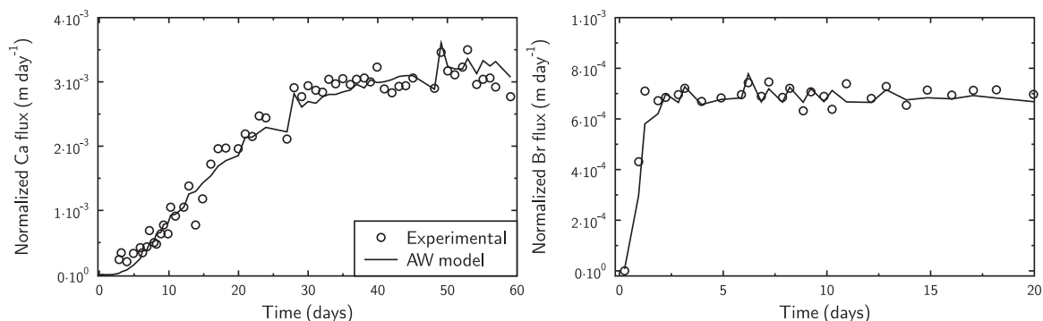
Fig. 12. Ca (left) and Br (right) mass flux densities as a function of time: experimental data (open circles) and AW model (full lines). See Fig. 1 for a description of the model and Table 3 for model parameters.
