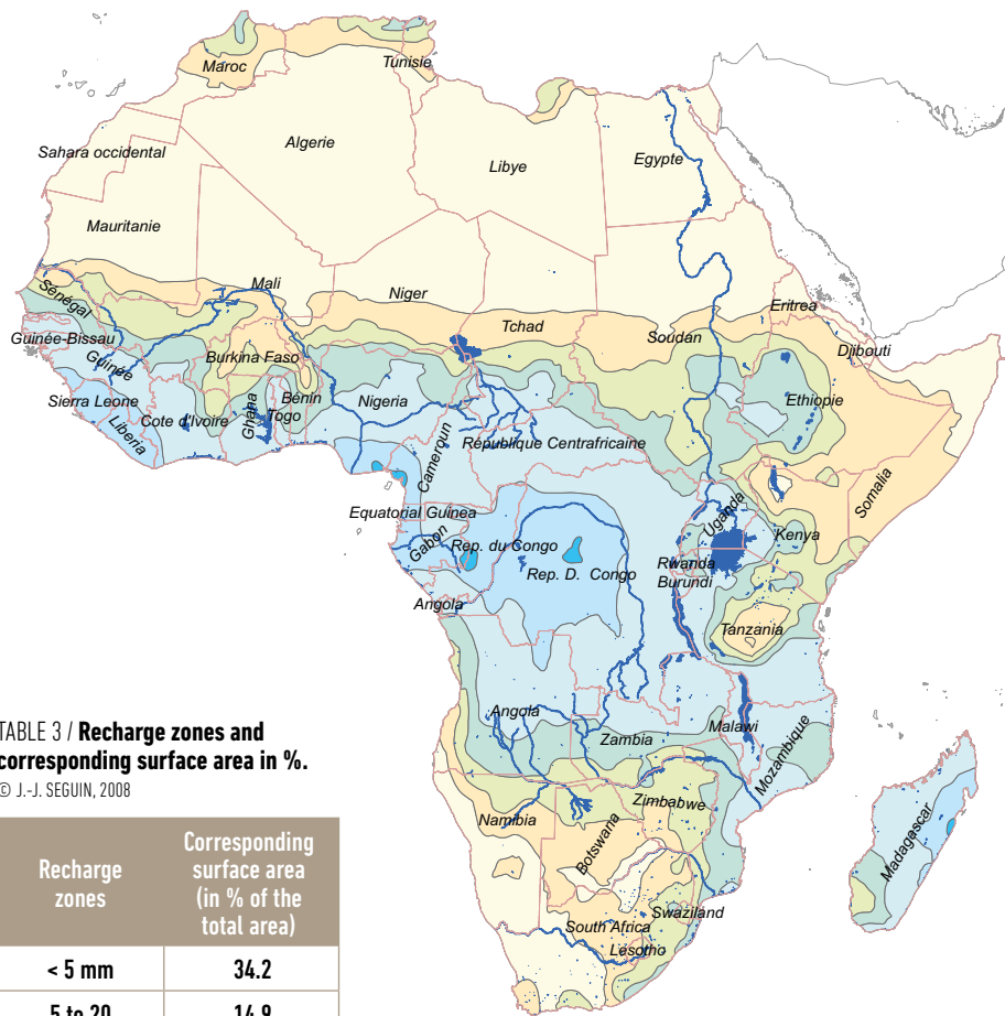
FIGURE 2 / Delimitation of seven recharge zones (according to the 1:10,000,000 hydrogeological map of Africa where the recharge results from an interpolation of a grid of values provided by P. Döll, 2005). © BRGM
