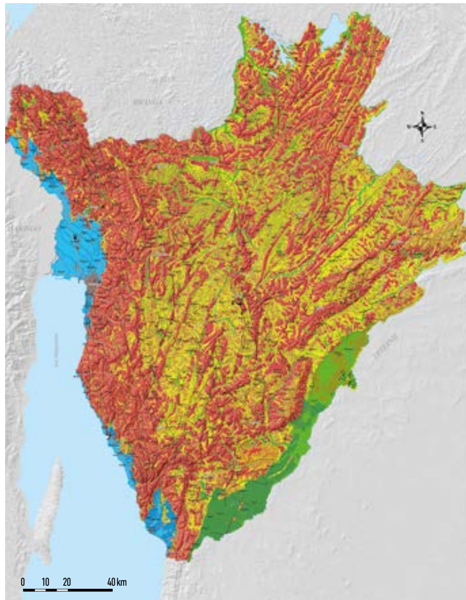
Map of groundwater potential in Burundi. © BRGM
