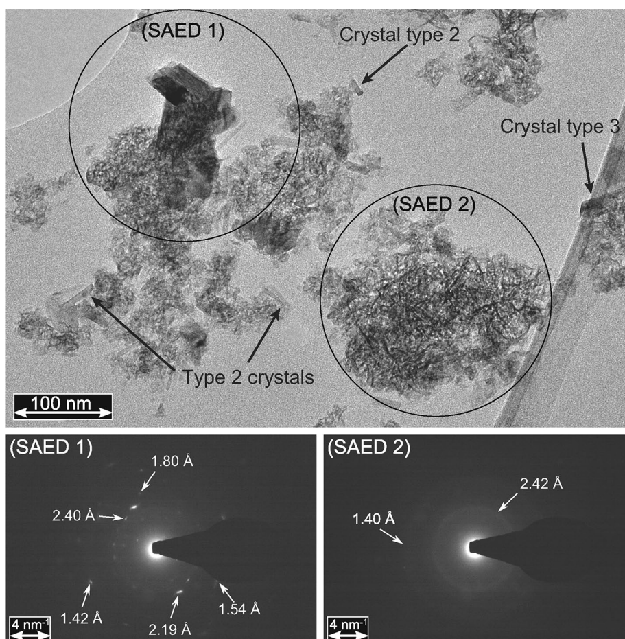
Fig. 8 TEM observation of \text{Mn}\delta\text{Bi}_3\text{-10y} and SAED patterns of type 1 and type 4 crystals. Top panel Low-magnification view of crystals from \text{Mn}\delta\text{Bi}_3\text{-10y} . Circles indicate areas which were subjected to electron diffraction. Circle at the top left (SAED 1) targeted crystal type 4, which had a diffraction pattern exhibiting features characteristics for cryptomelane, and in particular d -spacing of 2.40, 2.19, 1.80, 1.54 and 1.42 Å (pattern at the bottom left). Circle at the bottom right (SAED 2) targeted crystal type 1 and had a signal typical for \delta\text{-MnO}_2 , with distances of 2.42 and 1.40 Å (pattern at the bottom right). Crystals types 2 and 3 which are most easily distinguishable are pointed out with arrows
