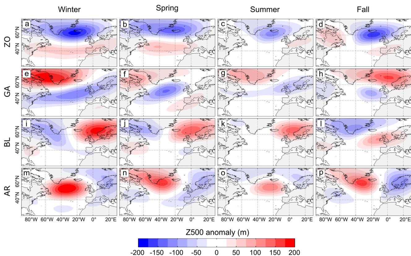
Fig. 3 North Atlantic weather regime centroids for winter (December, January, February), spring (March, April, May), summer (June, July, August) and fall (September, October, November). The centroids are computed from the anomaly maps of the 500-hPa geopotential height
