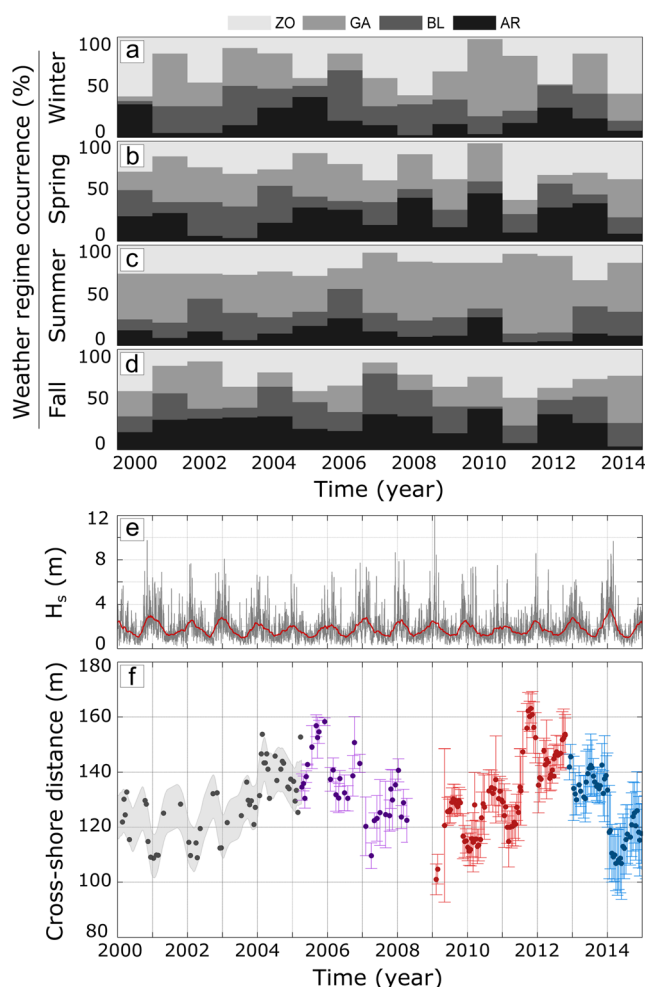
Fig. 2 a–d Seasonal weather regime occurrence in percentage derived from the ERA-Interim reanalysis from winter 2000 to fall 2014. ZO , GA , BL and AR Zonal, Greenland anticyclone, blocking and Atlantic ridge regimes, respectively. e Significant wave height H_s and 90-day moving average (red line). f Measured shoreline position using the mean high water level proxy at z=1.5 m. Gray dots Shoreline positions calculated using single beach profiles, colored dots shoreline positions calculated by averaging the position of the mean high water level iso-contour over an alongshore distance of approx. 350 m (purple), 750 m (red) and 1,500 m (blue). Error bars Associated cross-shore standard deviation. Gray area 90-day moving average \pm mean cross-shore standard deviation
