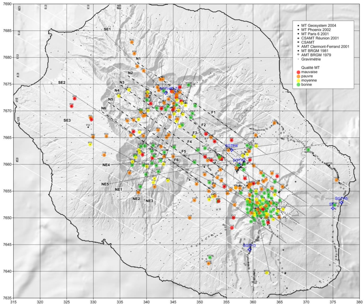
Figure 3: Map of the quality of resistivity data.
