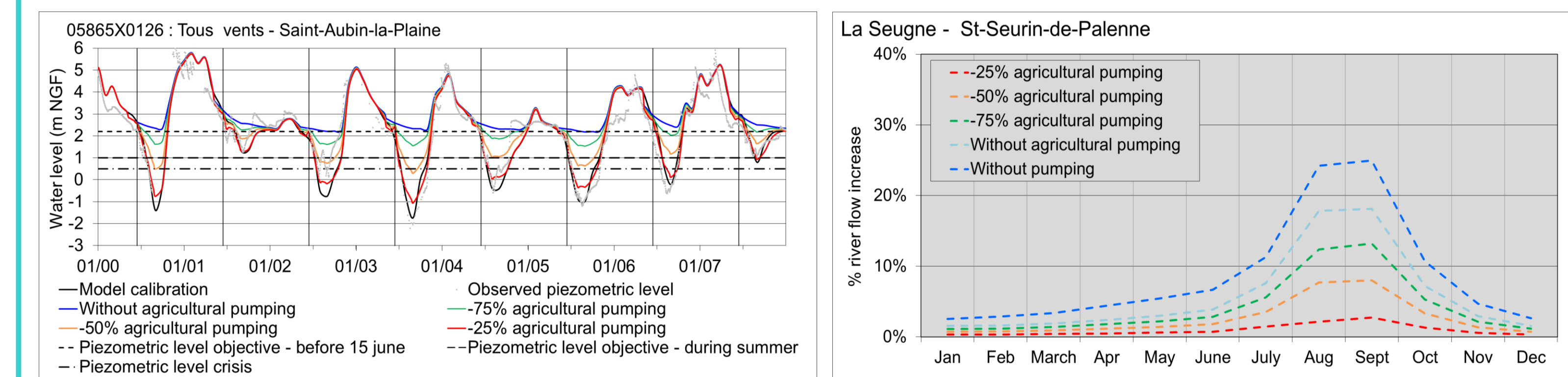
Water level depending on different pumping down scenario and objective level - Jurassic model (b) Flow increase versus lower pumping - Interannual monthly average of 2000-2008 - Cretaceous model (c)
