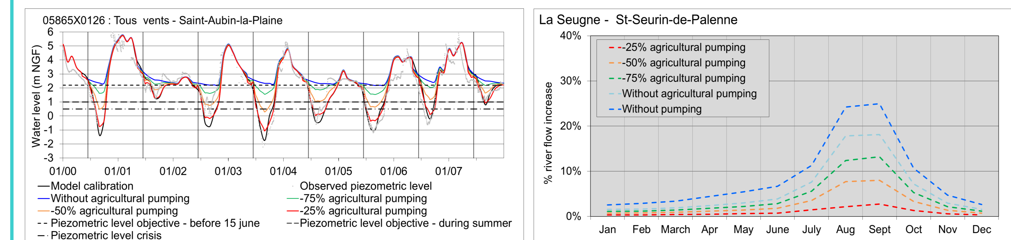
Water level depending on different pumping down scenario and objective level - Jurassic model (b)
