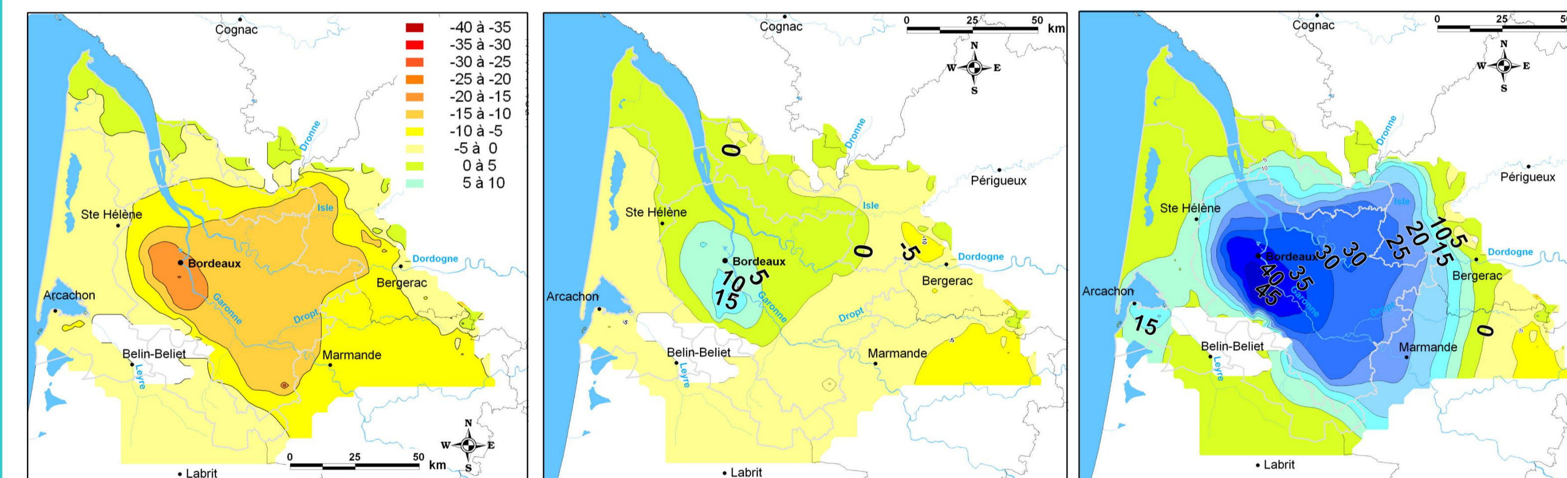
Simulation with current pumping trend (e) Simulation with pumping scenarios (pumping in others areas / aquifers) (e) Simulation without pumping (e)
