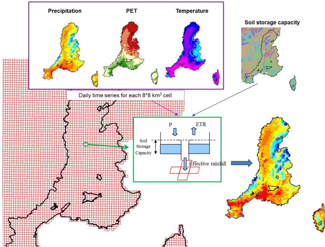
Figure 1: Methodological sketch of the gridded water budget method for effective rainfall computation (here applied over the whole Rhône-Mediterranean & Corsica basin, see figure 2).
