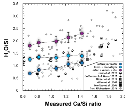
Figure 1. Plots of \text{H}_2\text{O}/\text{Si} against \text{Ca}/\text{Si} with the gray diamonds are adapted from 5. The blue circles are for interlayer water, the light blue ones for interlayer water and a single adsorbed monolayer and the purple ones are with the contribution of hydroxyls from this work.
