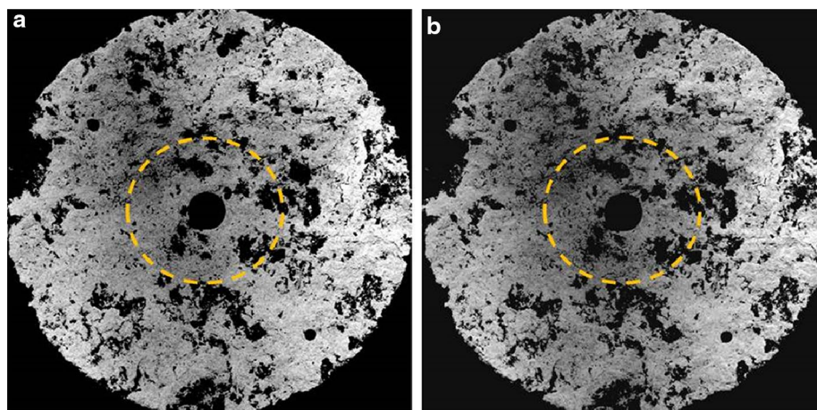
Fig. 20 X-ray microfluorescent maps of the calcium. In the lower wall before (a) and after (b) the percolation test (black shows the absence of calcium)
