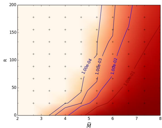
Figure 7 : Graphical representation of P(DS|\tilde{M}, \tilde{R}) .
