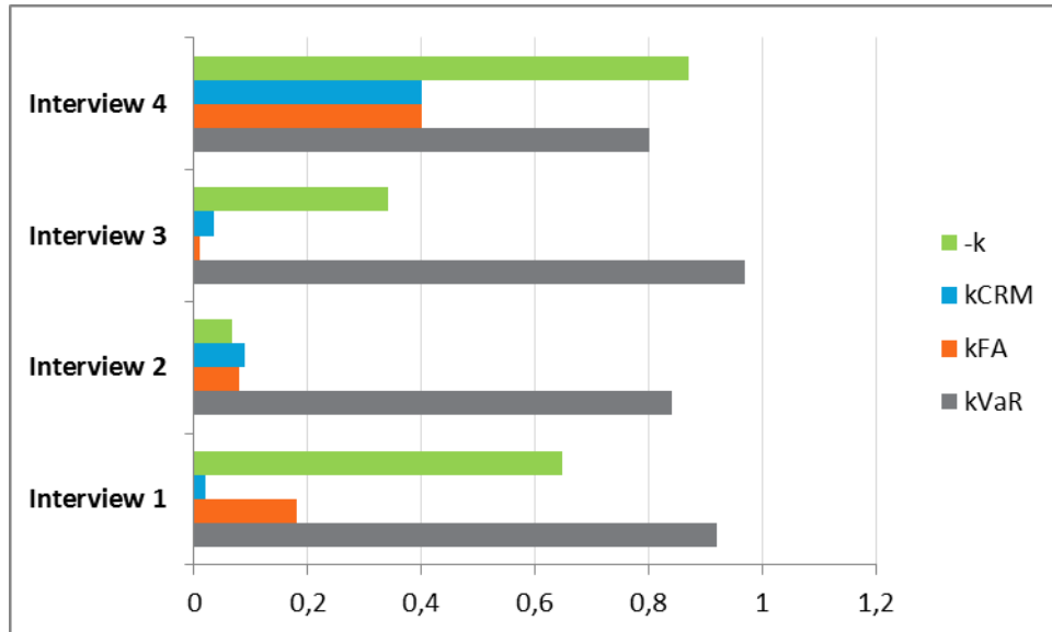
Figure 15 : Comparison of the constants of the global utility function from the four interviews
