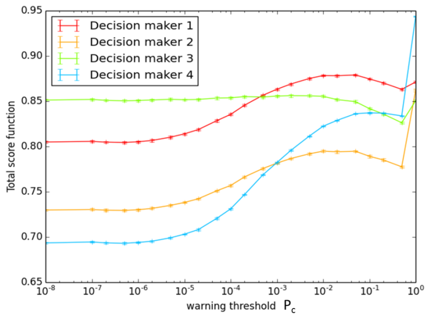
Figure 10 : Expected value of the score function depending on the warning threshold, with preferences from the four DMs (error bars correspond to the 95% confidence intervals).
