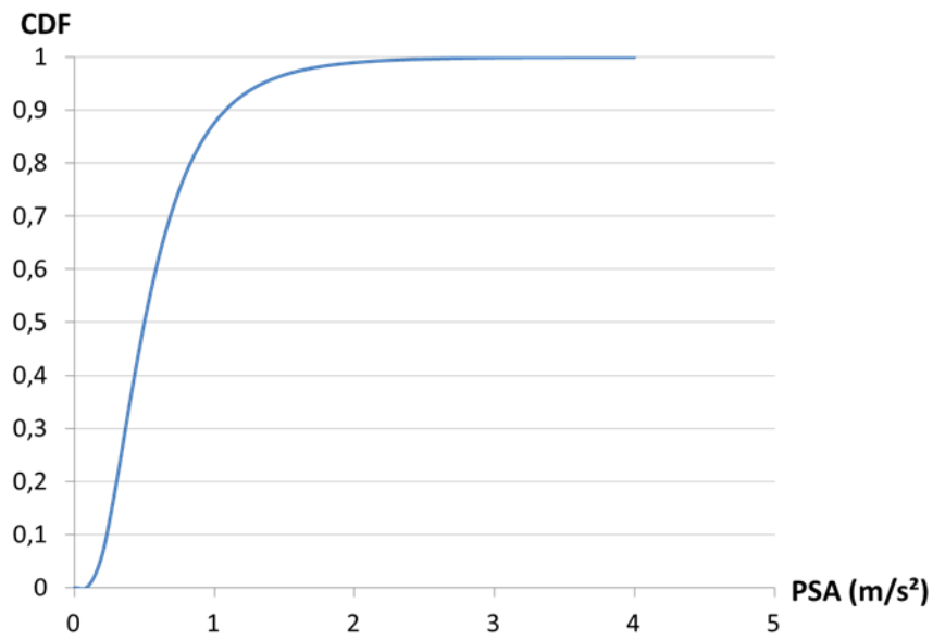
Figure 5 : Fragility curve for the hypothetical bridge (corresponding to DS3) (PSA: peak spectral acceleration; CDF: cumulative distribution function)
