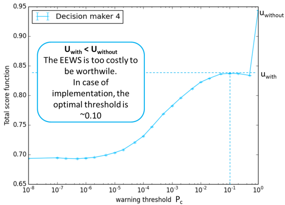
Figure 12 : Expected value of the global utility function depending on the warning threshold for DM n°4.
