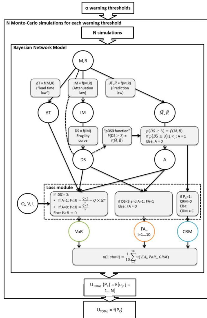
Figure 3 : Bayesian network used for the case study.
