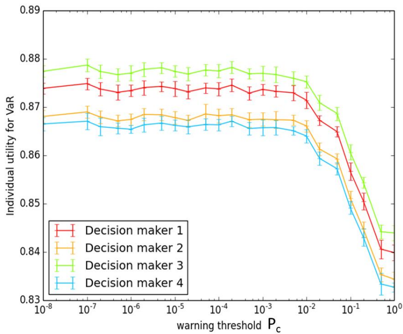
Figure 13 : Expected value of U_{\text{VaR}} depending on the warning threshold, with preferences from the four DMs (error bars correspond to the 95% confidence intervals).
