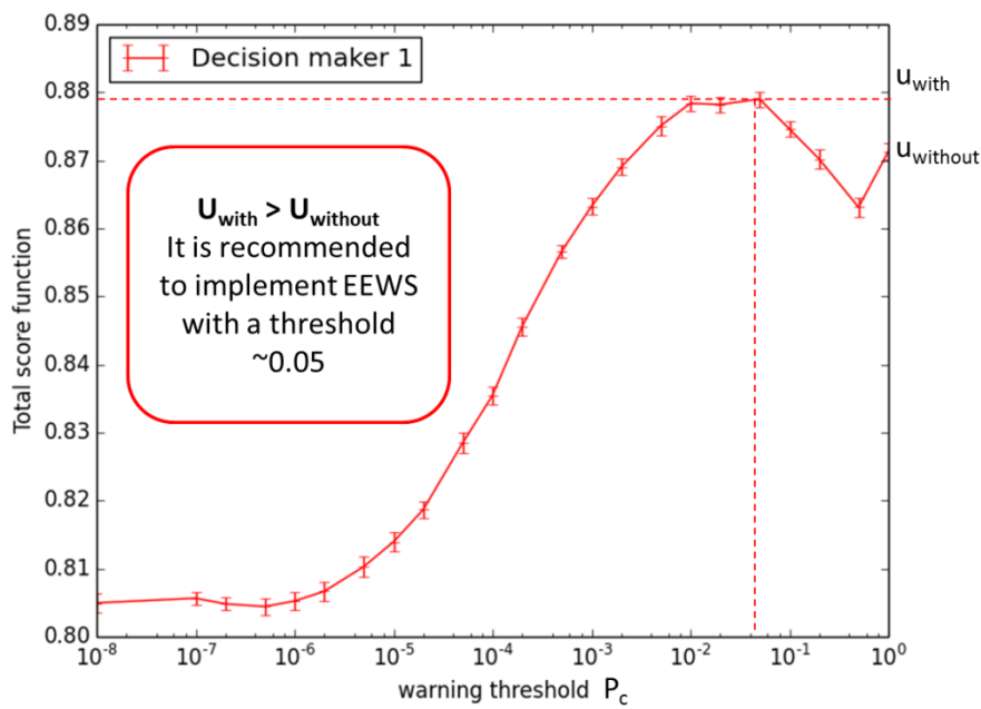
Figure 11 : Expected value of the global utility function depending on the warning threshold for DM n°1.
