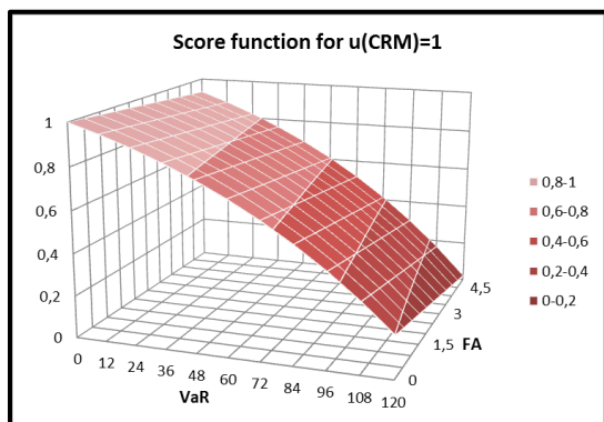
Figure 9: Graphical representation of the global utility function for DM n°1.
