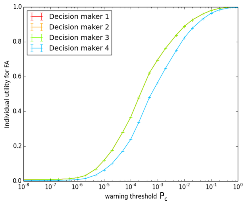
Figure 14 : Expected value of U_{FA} depending on the warning threshold, with preferences from the four DMs. The first three curves are identical (Error bars correspond to the 95% confidence intervals).
