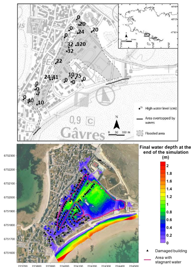
Figure 10. Above: measurements of maximum water depths (modified from Cariolet, 2010); below: final water depth at the end of the SURF-WB simulation and reported flooded buildings and stagnation area according to the municipality (from the Gâvres municipality and Le Cornec and Peeters, 2008).
