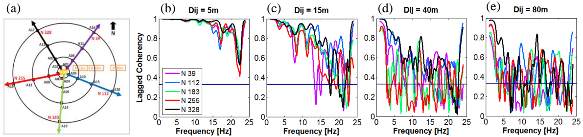
Figure 3. (a) Array configuration. (b)-(e) Lagged coherency of the EW component of the event for pairs lying in 5 array-branch directions and at 4 separation distances.
