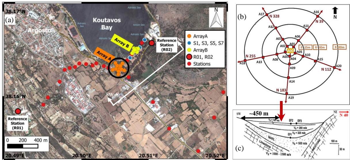
Figure 1. (a) Location and (b) layout of Array A in the seismological experiment at Argostoli. (c) 2D model of the SW-NE cross-section of the Argostoli valley (Protopapa et al. , 1998). The red arrow points out the location of Array A.
