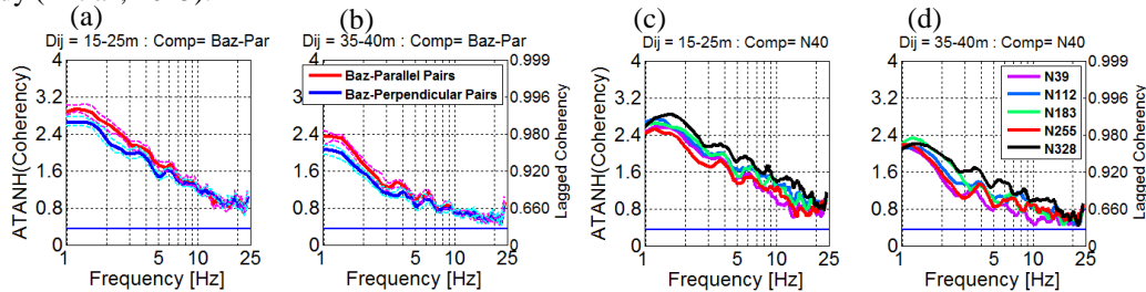
Figure 6. Comparison of ATANH coherency between the event back-azimuth oriented station pairs at separation distances (a) 15-25 and (b) 35-40 m for the baz-parallel horizontal component. Red and blue curves indicate the two groups of pairs while magenta and cyan curves indicate the respective 85% CI intervals. Comparison of ATANH coherencies among the five array-branch directions at separation distances (c) 15-25 and (d) 35-40 m for valley-perpendicular (N40) horizontal component. Blue straight line marks the coherency resolvability threshold. The corresponding lagged coherency values are marked at the right-side axis of the figure.
