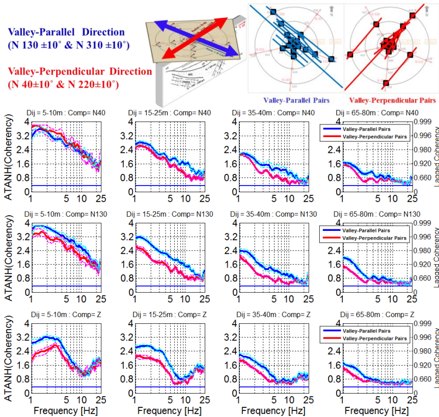
Figure 7. Comparison of ATANH coherencies between the valley-perpendicular and valley-parallel station pairs, for valley-perpendicular ( N40 ), valley-parallel ( N130 ) and Z horizontal components. Red and blue curves indicate the two groups of pairs while magenta and cyan curves indicate the respective 85% CI intervals. The corresponding lagged coherency values are marked at the right-side axis of the figure. D_{ij} stands for interstation distance, Comp for the component of ground motion. Blue straight line marks the coherency resolvability threshold. On top, the two station-orientations and the respective pairs are schematically explained.
