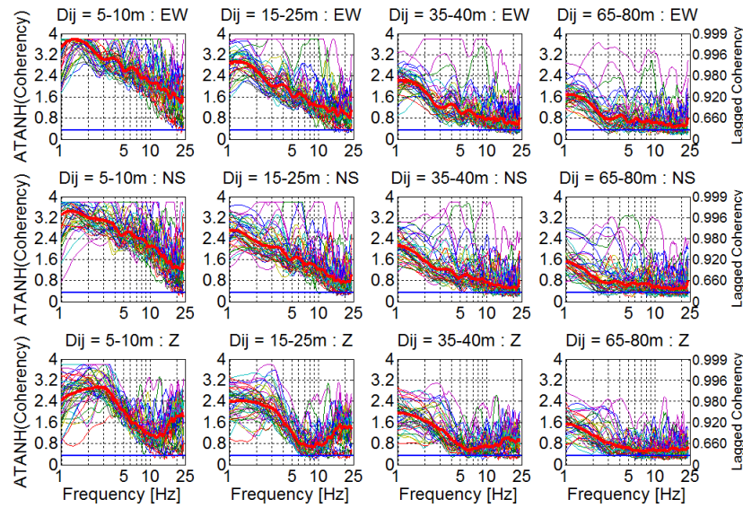
Figure 4. Median estimates of ATANH coherency of 46 events at four separation distances. The corresponding lagged coherency values are marked at the right-side axis of the figure. The thick red curve shows the ‘global median’. Dij stands for interstation distance and EW, NS, Z for the ground-motion components. Blue straight line marks the coherency resolvability threshold.
