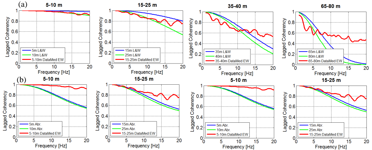
Figure 8. Comparison of the global lagged coherency of Argostoli data with (a) the analytical model of Luco and Wong (1986) and (b) the empirical model of Abrahamson (1991) for the EW component and at 4 separation distances. The blue and green curves show the estimates given by the parametric models and the red curve shows the global median estimate from the Argostoli array data.
