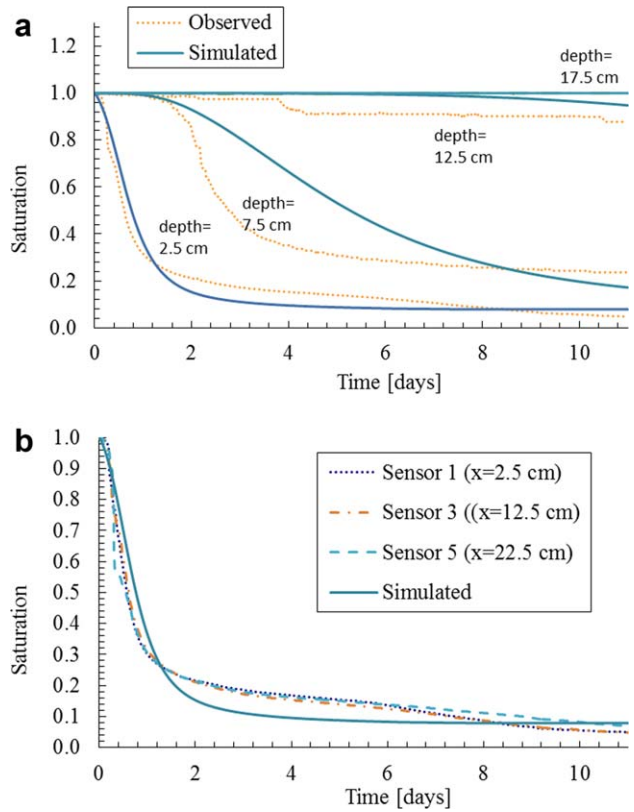
Figure 24. Comparison between experimental and theoretical saturation results for U = 1.2 \text{ m/s} at (a) x = 0.125 \text{ m} and (b) depth of 0.025 m.
