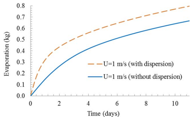
Figure 12. Comparison between evaporation processes with and without taking dispersion in the free-flow domain into account ( K = 1 \times 10^{-10} \text{ m}^2 , S_{wr} = 0.075 , U = 1 \text{ m/s} , T_U = 313 \text{ K} , w_{v,U} = 0.006 , \alpha_{BJ} = 0.01 , \phi = 0.33 ).
