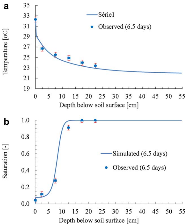
Figure 25. Simulated and observed (a) temperature and (b) saturation at t = 6.5 \text{ days} for soil profile at tank center (arc-length 0.125 m).
