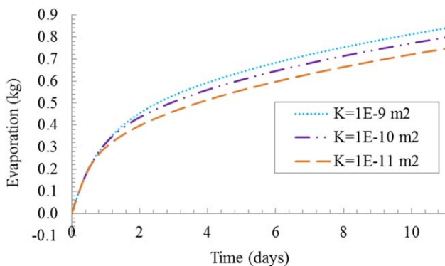
Figure 19. Effect of porous medium permeability on drying process ( S_{wr} = 0.075 , U = 1 \text{ m/s} , T_U = 313 \text{ K} , w_{vU} = 0.006 , \alpha_{BJ} = 0.01 , \phi = 0.33 ).
