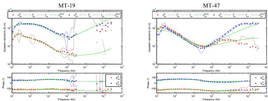
Figure 4 : MT soundings 19 (left) and 47 (right) showing data (off-diagonal components in red and blue) and model responses in green. Upper plots display the resistivity and lower plots the phase for the same components.
