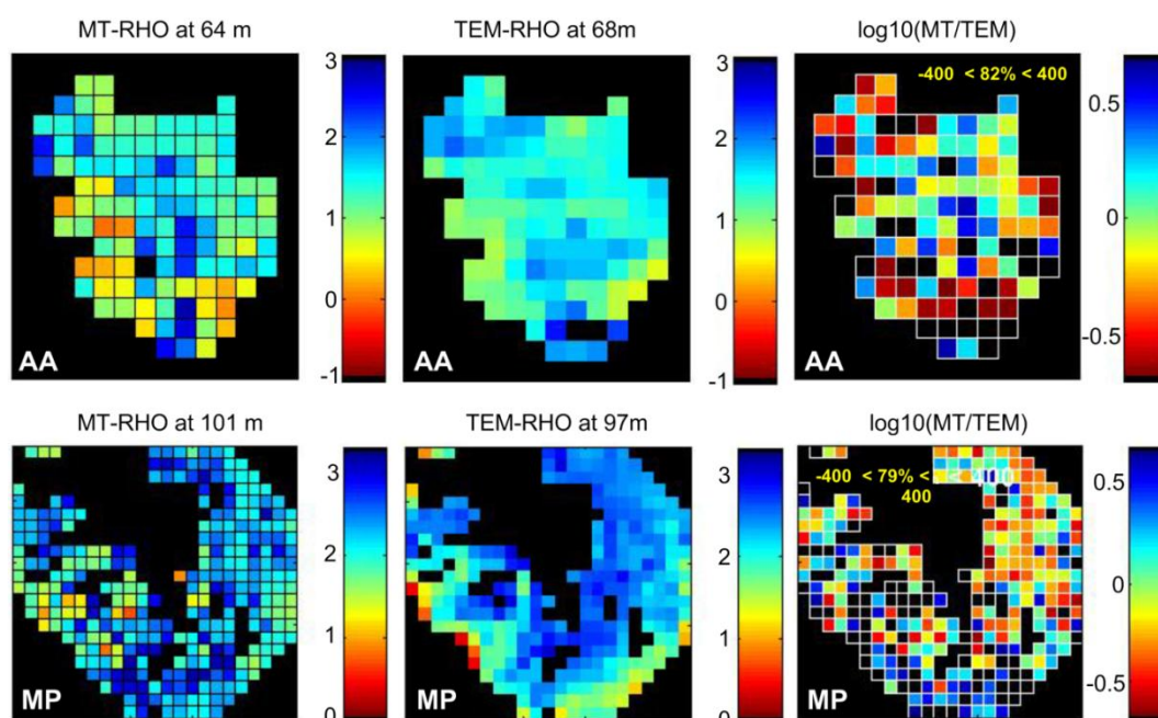
Figure 7 : MT versus TEM resistivity for superficial layers. Above are represented the data of the Ansed'Arlet (AA) geothermal province and below from the MontagnePelée (MP) geothermal province. Left plots display resistivity from the 3-D MT models for both sector at the indicated depth. Center plots display resistivity of the TEM data (see text for details). Right plots show variation between the two models (log scale).
