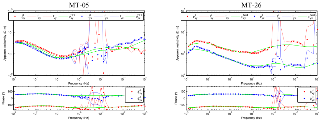
Figure 1: MT soundings 05 (left) and 26 (right) showing data (off-diagonal Z_{xy} and Z_{yx} components in red and blue, respectively) and model responses in green. Upper plots display resistivity and lower plots phase for the same components.
