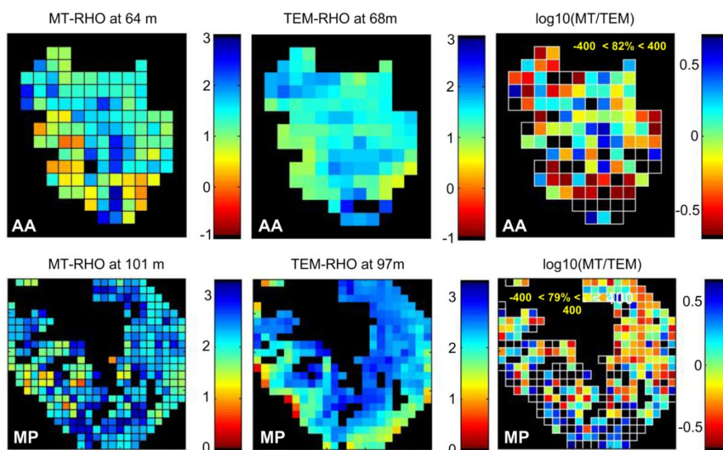
Figure 7 : MT versus TEM resistivity for superficial layers. Above are represented the data of the Ansed'Arlet (AA) geothermal province and below from the MontagnePelée (MP) geothermal province. Left plots display resistivity from the 3-D MT models for both sector at the indicated depth. Center plots display resistivity of the TEM data (see text for details). Right plots show variation between the two models (log scale).
