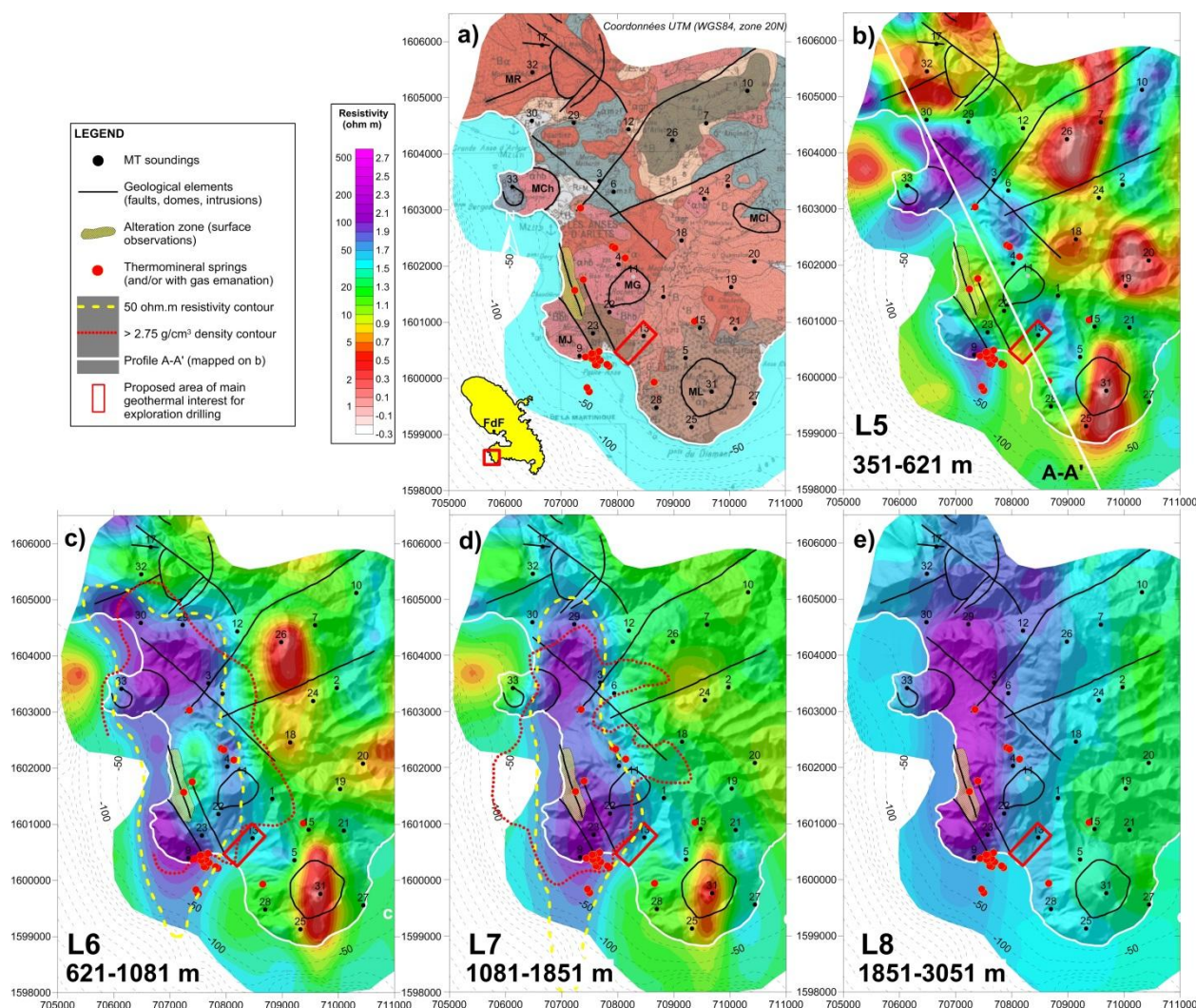
Figure 2 : a) Location map of the investigated area on geological background (Westercamp et al. 1900) and resistivity models at 351 to 3051mdeep(b, c, d, e). Superimposed elements are indicated in the legend.
