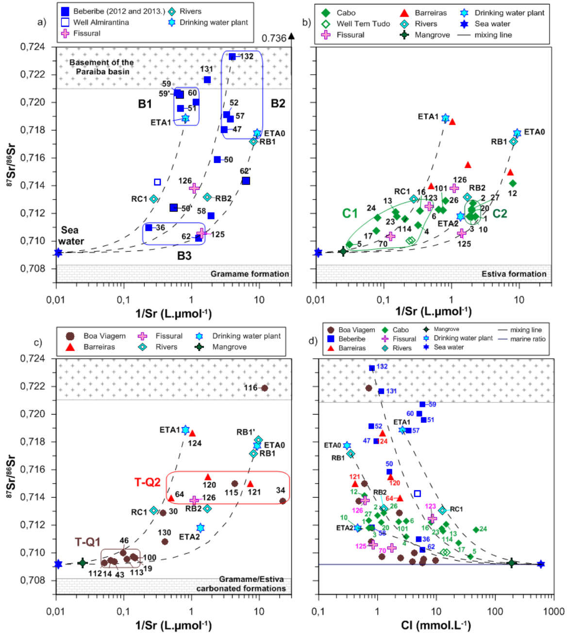
Figure 6: a) 1/\text{Sr} (L.mol -1 ) vs. strontium isotopes in a) the Beberibe, b) Cabo, c) Barreiras and Boa Viagem aquifers, and d) Cl concentrations vs. strontium isotopes in the sampled groundwater of the study area. Data from rock samples, i.e. from the basement of the Paraíba basin (Brito Neves, 1975) and from the Gramame formation (Nascimento-Silva et al., 2011) are also indicated. Errors are within the point. Dashed lines represent mixing of seawater with surface waters considered as recharge (ETAs).
