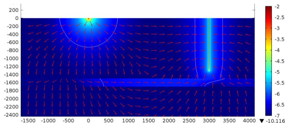
Figure 2: Electrical current density (log scale, A/m 2 ) below a surface injection (left) and when using a metallic casing (right side, down to 1300 m here) for 2 Hz current injection. The current flows preferably at depth all along the borehole and particularly in the conductive layer. The ratio target response versus primary source is more favorable with the casing injection.
