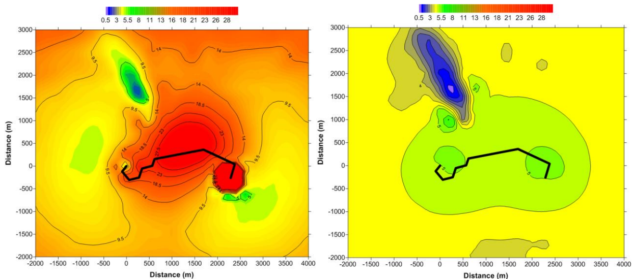
Figure 4: Left, 8 Hz in-phase electric field amplitude converted in a highly distorted apparent resistivity map (in Ohm.m) using a pure geometric factor (DC assumption). Right after a normalization based on the computation of the EM field at 8 Hz over a homogeneous medium at 5 Ohm.m, the anomaly is well resolved with few artifacts.
