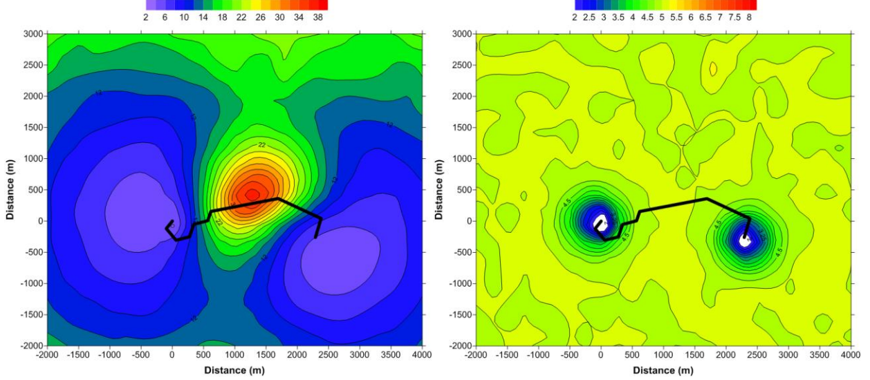
Figure 5: 8 Hz in-phase electric field converted in apparent resistivity map (no anomaly here, only homogeneous medium at 5 Ohm.m). Left, error introduced when normalizing with the exact geometry but with a DC assumption at 5 Ohm.m. Right, error introduced when normalizing by surface electrode response (instead of 450 m long boreholes) calculated at 8 Hz over a 5 Ohm.m ground.
