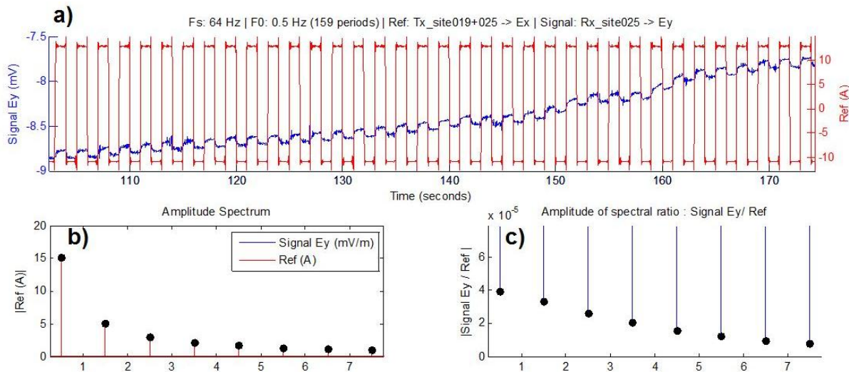
Figure 1: Example of CSEM data processing for an electric channel: a) time serie of injected current (~7 A) and recorded signal for a 200 m length dipole, b) frequency spectrum for Current c) modulus of ratio E/I. Black dots indicate data at measuring frequencies (here : 0.5 Hz, 1.5 Hz, etc...)
