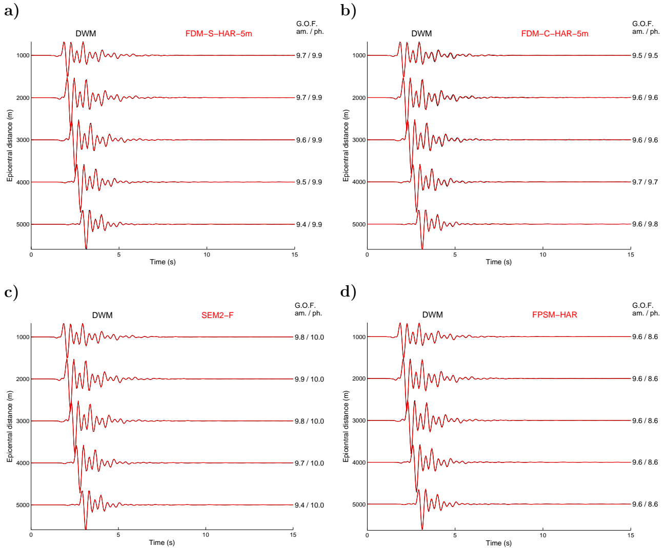
Figure 17. East-West component of ground velocity along the northern surface profile computed for the 1D-smooth case by 4 different methods: a) FDM-S; b) FDM-C; c) SEM2-F; d) FPSM.
