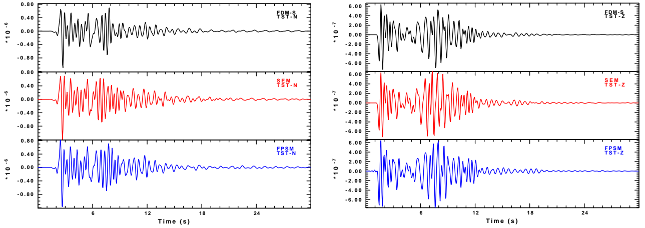
Figure 2. Comparison of predictions of the NS (left) and vertical (right) components of ground velocity at the central TST station obtained by three different numerical methods: FDM-S (black), SEM (red) and FPSM (blue). The sedimentary basin is modeled with three homogeneous visco-elastic layers of varying thicknesses described in Fig. 1 and Table 1.
