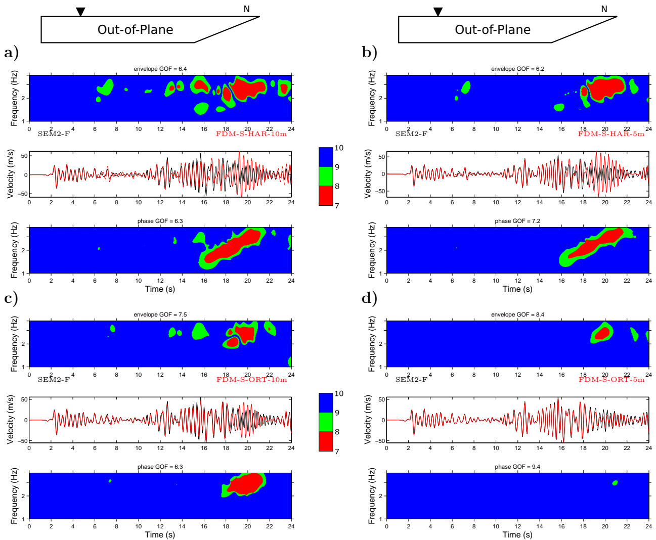
Figure 28. Same as Fig. 27 for solutions computed with FDM-S using different grid spacings and definitions of the effective medium: a) harmonic averaging, 10 m; b) harmonic averaging, 5 m; c) orthorhombic averaging, 10 m; d) orthorhombic averaging, 5 m.
