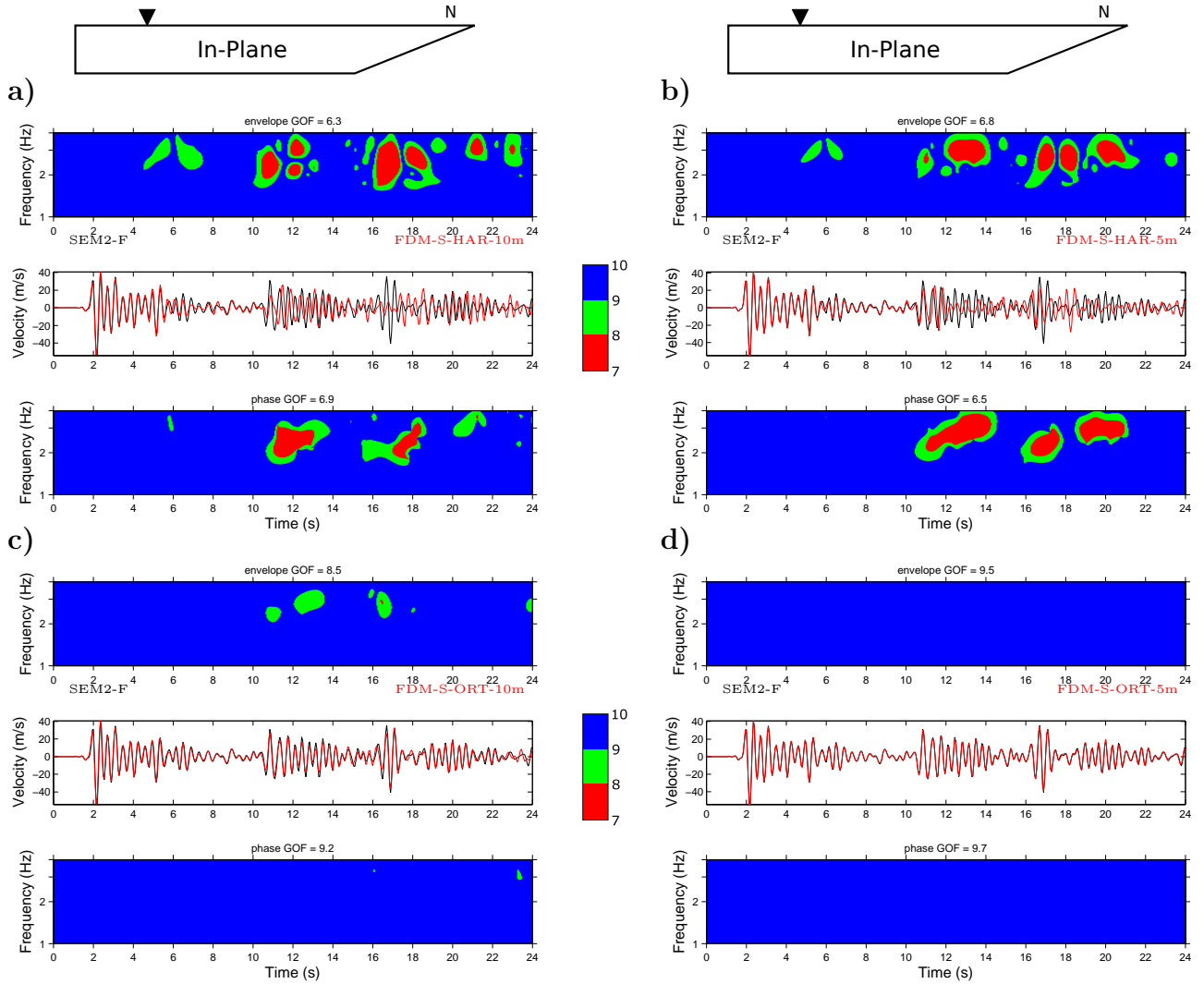
Figure 25. Same as Fig. 24 for solutions computed with FDM-S using different grid spacings and definitions of the effective medium: a) harmonic averaging, 10 m; b) harmonic averaging, 5 m; c) orthorhombic averaging, 10 m; d) orthorhombic averaging, 5 m.
