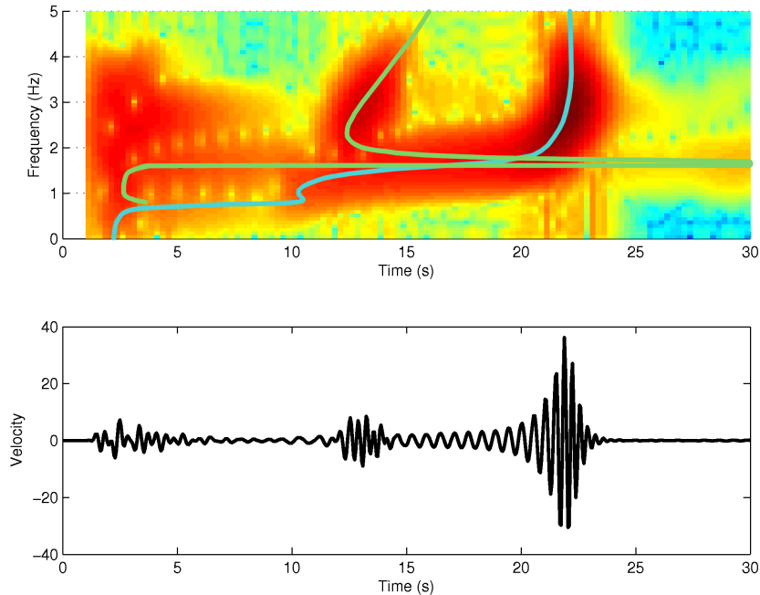
Figure 10. Same as Fig. 8 for the 1D-smooth case.
