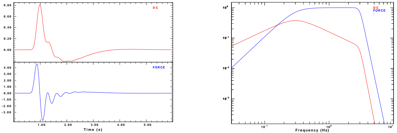
Figure 6. Source time functions used in the test cases 1D-sharp and 1D-smooth. Left: dimensionless time histories for the deep double-couple source (red) and the surface force (blue). Right: corresponding amplitude Fourier spectra.
