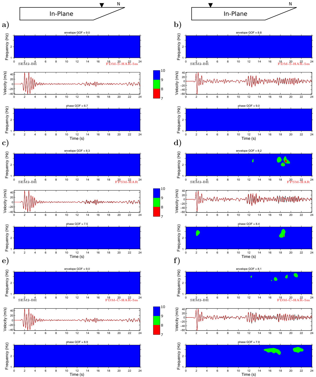
Figure 30. North-South component of ground velocity at receivers along the western surface profile of Fig. 11, 1 km away from the northern (left) or southern (right) edge, computed for the 2D-smooth case by three teams using a-b) FDM-S, c-d) FPSM, e-f) FDM-C. The SEM2-BE solution is taken as a reference and is plotted in black. The level of agreement between each solution and the reference is quantified by the time-frequency goodness-of-fit (GOF) in amplitude (top panel) and phase (bottom panel). The color scale indicates the level of GOF, from 7 to 10 (perfect fit). The average GOF is indicated on top of the time-frequency subplots.
