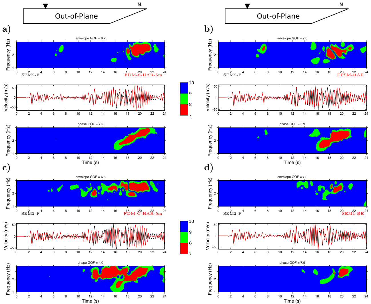
Figure 27. Same as Fig. 26 at a receiver 1 km away from the southern edge of the basin.
