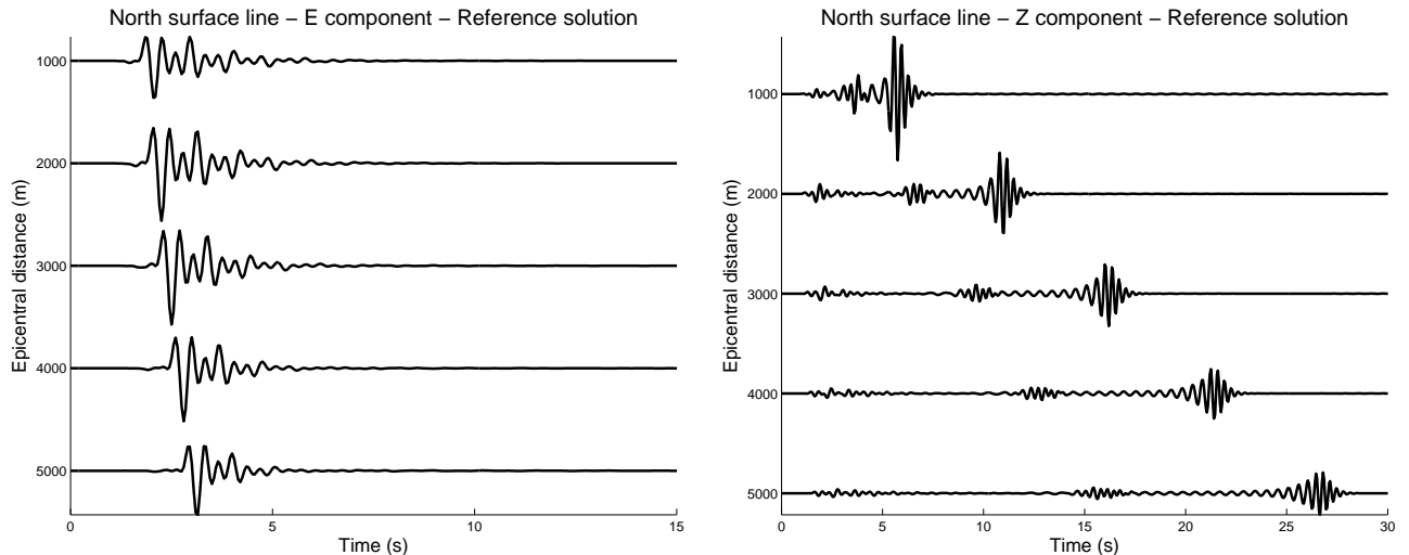
Figure 9. East-West (left) and vertical (right) components of ground velocity along the northern surface profile computed with the Discrete Wavenumber Method for the 1D-smooth model.
