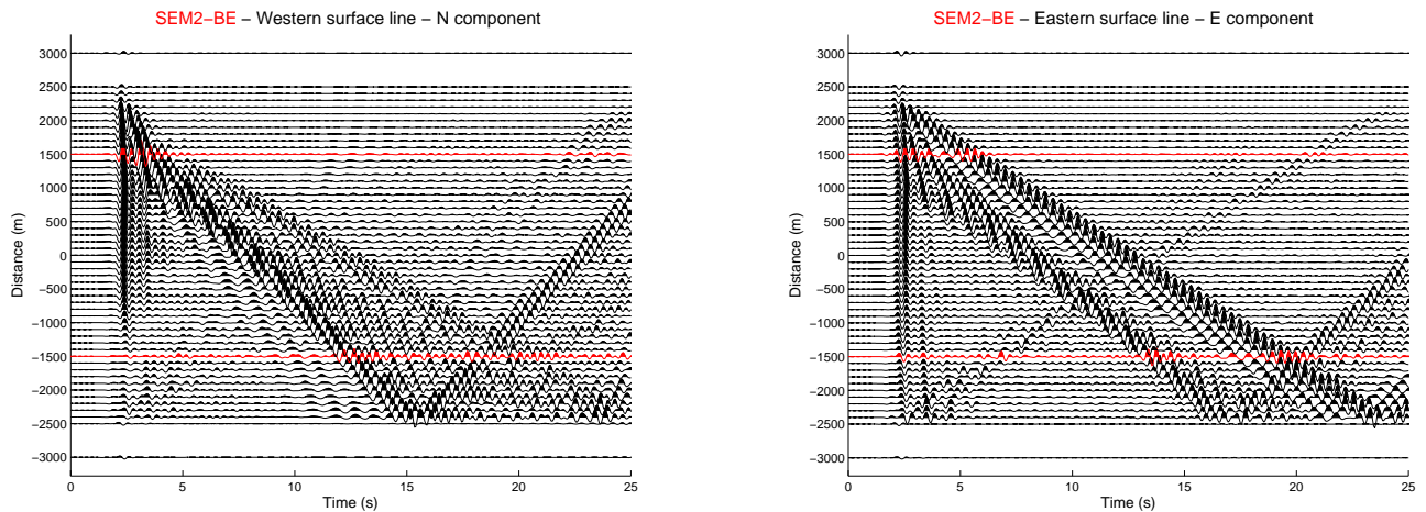
Figure 29. Seismic sections of the North-South (left) and East-West (right) components of ground velocity along the western (left) and eastern (right) profiles (Fig. 11) computed with SEM2-BE for the 2D-smooth case. The distance is measured from the centre of the valley and increases towards North. The left (resp. right) panel shows strong Rayleigh (resp. Love) wave trains excited at the northern edge. Red traces correspond to locations where the different numerical predictions are further compared.
