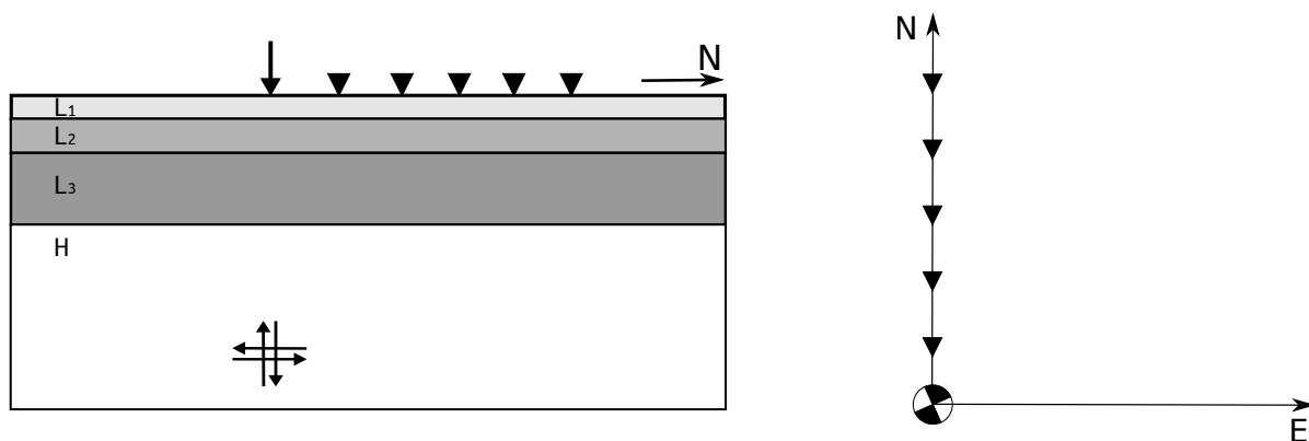
Figure 5. Schematic representation (left: vertical cross-section, right: surface view) of the 3 layers ( L_1 , L_2 , L_3 ) over halfspace ( H ) models used in the test cases 1D-sharp and 1D-smooth. The values of thicknesses, densities and seismic velocities are given in Tables 1 and 2. The positions of the sources and surface receivers are indicated with bold arrows and triangles, respectively. The beach ball at the epicentre indicates the focal mechanism of the double-couple point source plotted. The distance between the receivers along the northern surface profile is 1 km.
