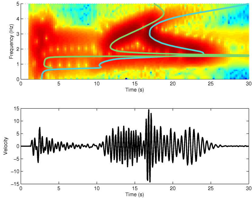
Figure 8. Time (bottom) and time-frequency (top) representations of the vertical ground velocity at 4 km epicentral distance for the 1D-sharp case. The background colours on the top image indicate the amplitude of the seismic arrivals, from blue (small) to red (medium) and bordeaux (large). The solid lines superimposed on the image indicate the theoretical group arrival times of the fundamental (blue) and first higher (green) modes of Rayleigh waves.
