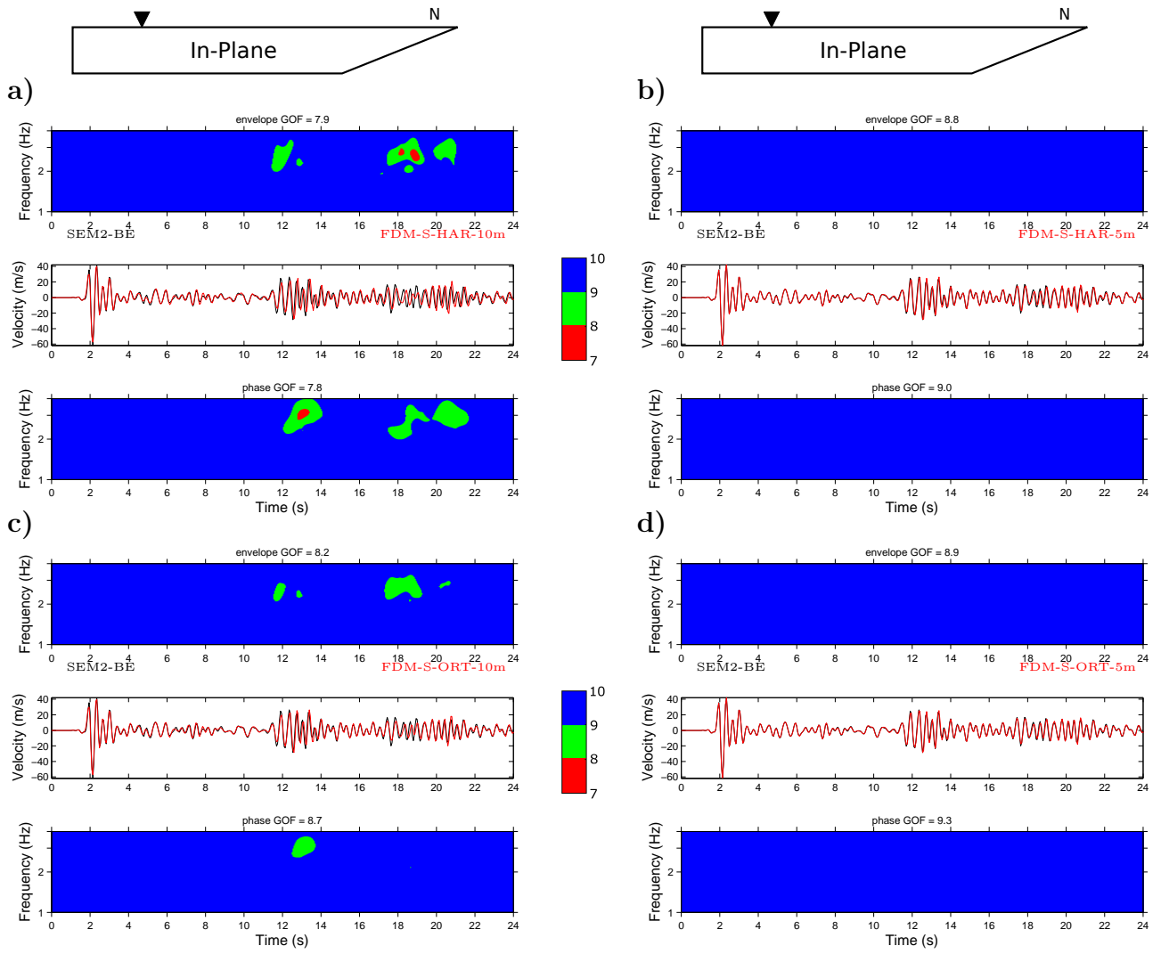
Figure 31. North-South component of ground velocity at the southern receiver for solutions computed with FDM-S using different grid spacings and definitions of the effective medium: a) harmonic averaging, 10 m; b) harmonic averaging, 5 m; c) orthorhombic averaging, 10 m; d) orthorhombic averaging, 5 m. The level of agreement between each solution and the reference is quantified by the time-frequency goodness-of-fit (GOF) in amplitude (top panel) and phase (bottom panel). The color scale indicates the level of GOF, from 7 to 10 (perfect fit). The average GOF is indicated on top of the time-frequency subplots.
