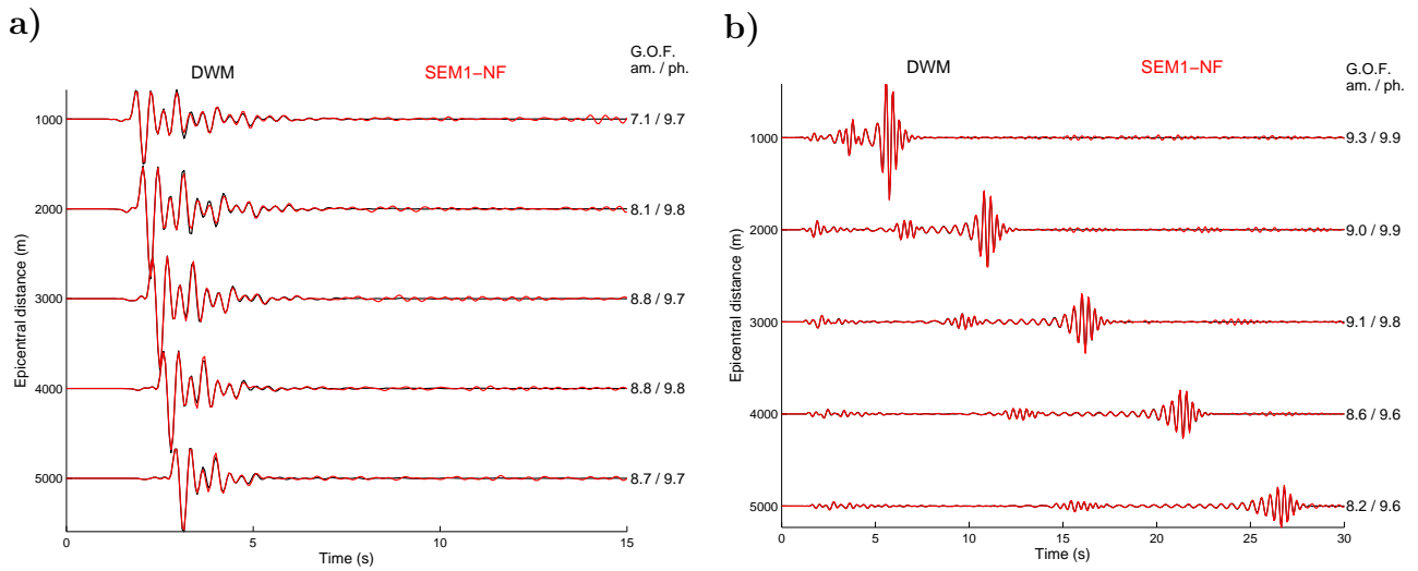
Figure 19. East-West (left) and vertical (right) components of ground velocity for the 1D-smooth case computed with SEM1-NF.
