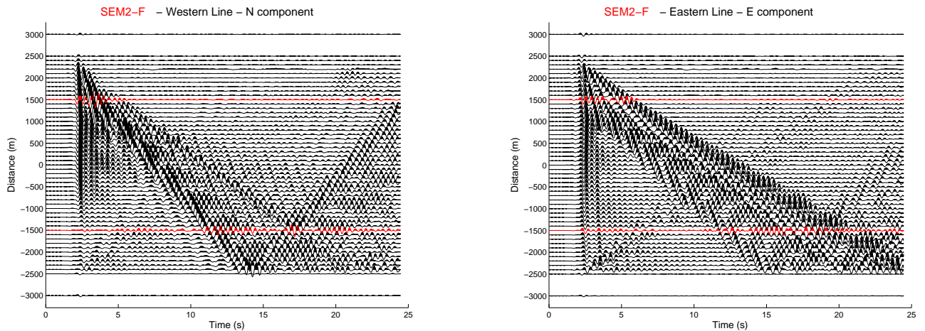
Figure 22. Seismic sections of the North-South (left) and East-West (right) components of ground velocity along the western (left) and eastern (right) profiles (Fig. 11) computed for the 2D-sharp case with SEM2-F. The distance is measured from the centre of the valley and increases towards North. The left (resp. right) panel shows a strongly dispersed Rayleigh (resp. Love) wave train excited at the northern edge. Red traces correspond to locations where the different numerical predictions are further compared (see text).
