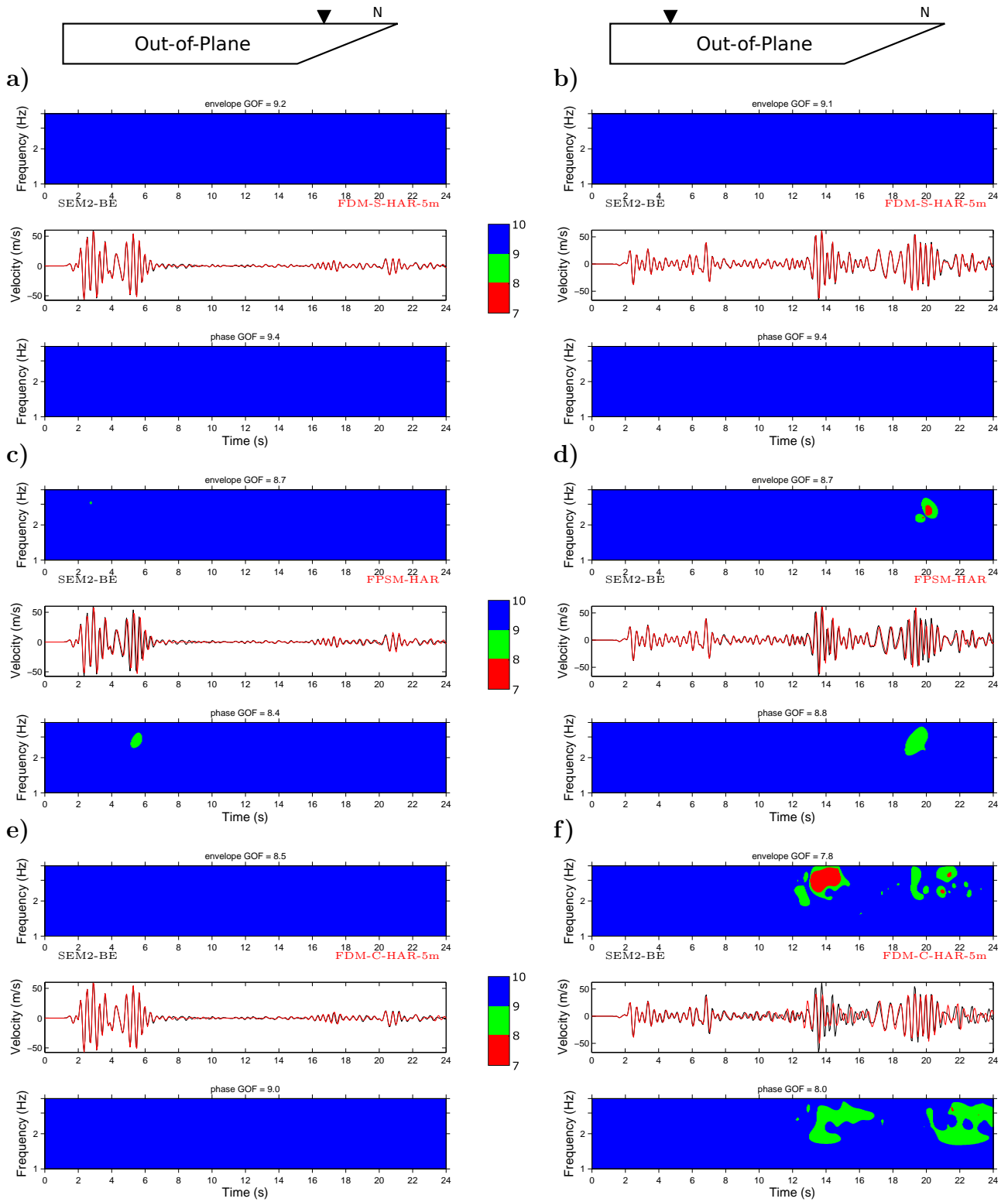
Figure 32. Same as Fig. 30 for the East-West component of ground velocity at receivers along the eastern surface profile of Fig. 11, 1 km away from the northern (left) or southern (right) edge.
