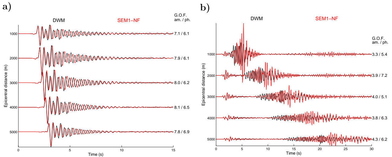
Figure 14. East-West (left) and vertical (right) components of ground velocity computed for the 1D-sharp case using SEM1-NF.
