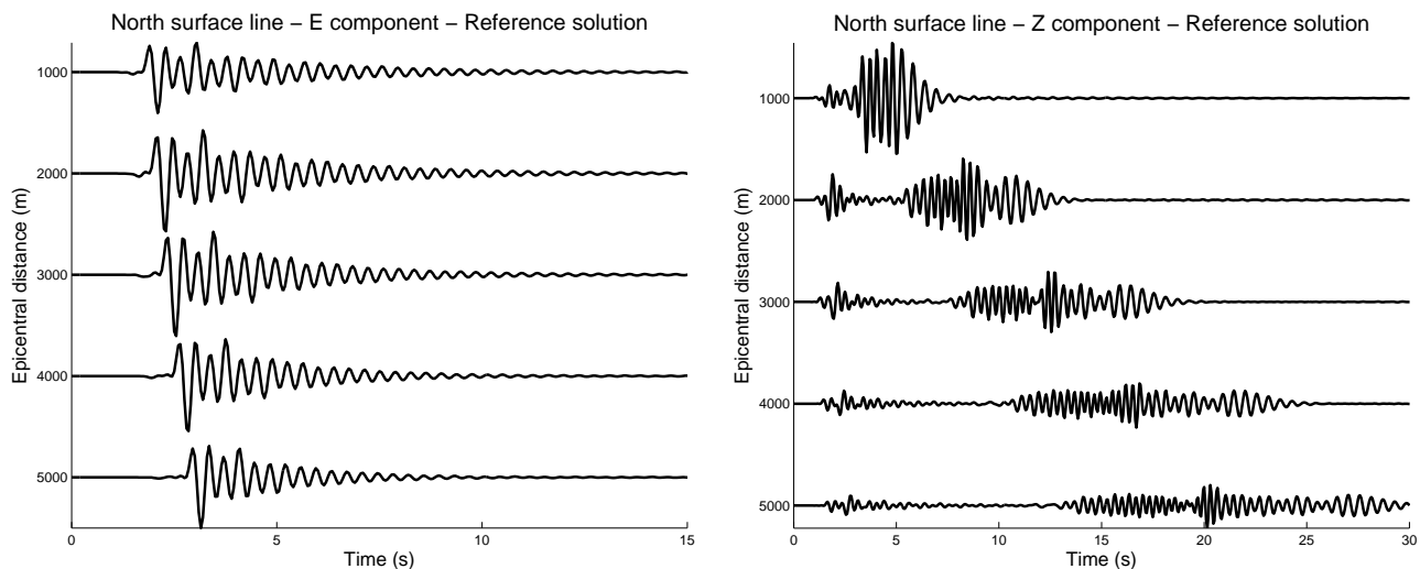
Figure 7. East-West (left) and vertical (right) components of ground velocity along the northern surface profile computed with the Discrete Wavenumber Method for the 1D-sharp model.
