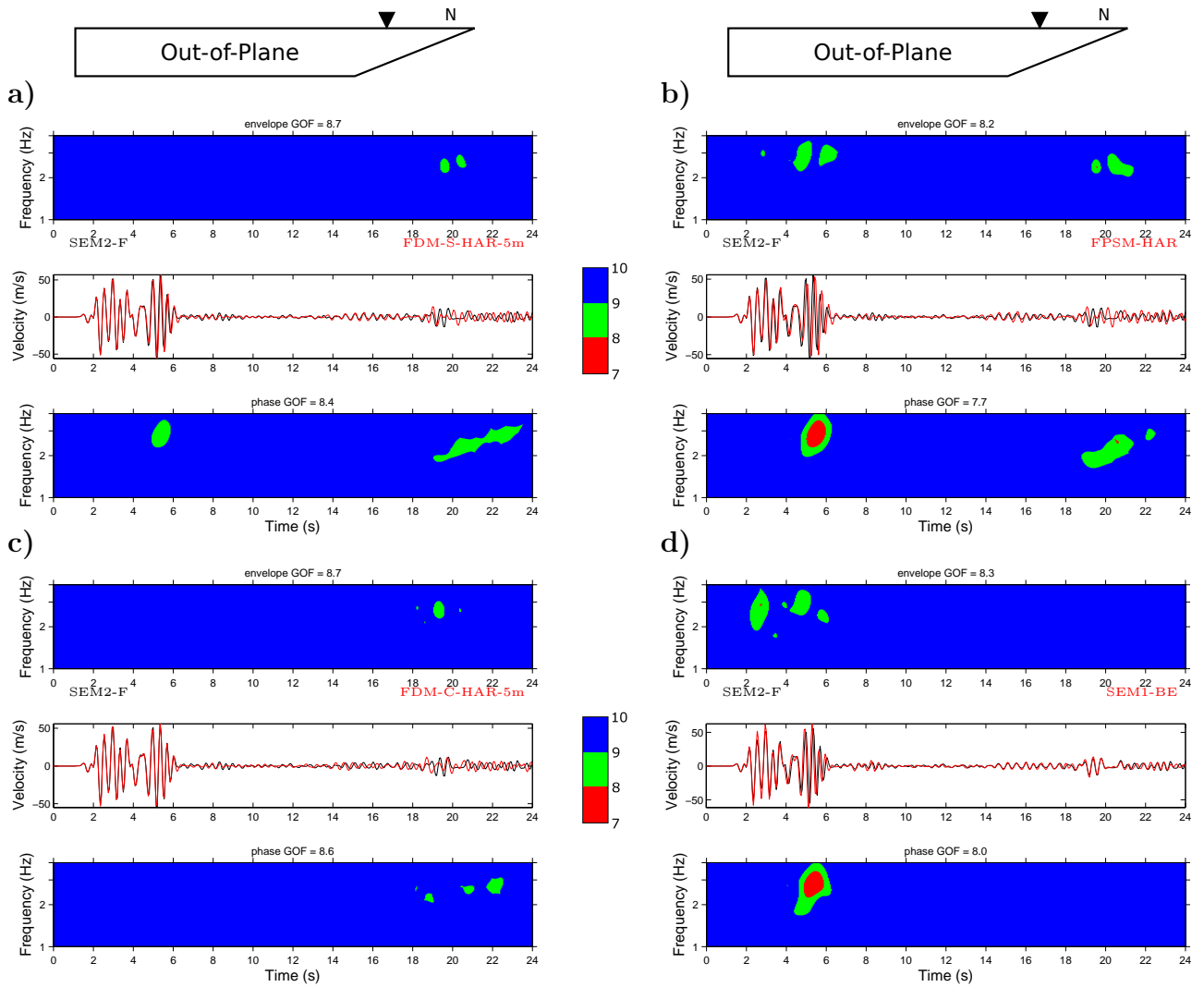
Figure 26. East-West component of ground velocity at a receiver along the eastern surface profile of Fig. 11, 1 km away from the northern edge, computed for the 2D-sharp case by a) FDM-S, b) FPSM, c) FDM-C, d) SEM1-BE. The SEM2-F solution is taken as a reference and is plotted in black. The level of agreement between each solution and the reference is quantified by the time-frequency goodness-of-fit (GOF) in amplitude (top panel) and phase (bottom panel). The color scale indicates the level of GOF, from 7 to 10 (perfect fit). The average GOF is indicated on top of the time-frequency subplots.
