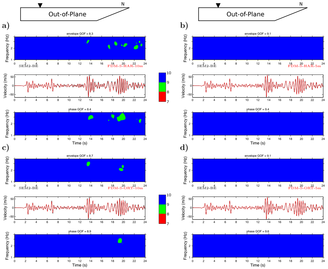
Figure 33. Same as Fig. 31 for the East-West component of ground velocity at the southern receiver.
