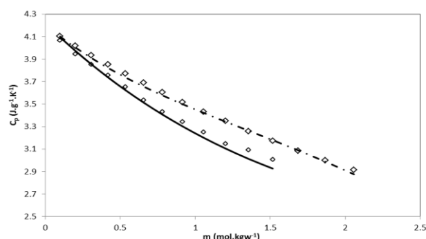
Fig. 3: Calculated (lines) and experimental (open symbols) heat capacity, C_p , for the \text{BaCl}_2\text{-H}_2\text{O} binary system as a function of \text{BaCl}_2 molality at 0°C (solid line) and 90°C (dash-dot line).
