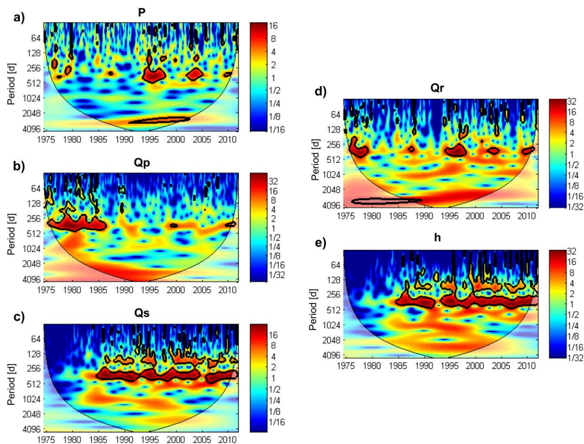
862 Figure 8: Continuous wavelet power spectra of the hydrogeological time series; the thick 863 black outline designates the 5% significance level against red noise and the cone of influence, 864 where edge effects might distort the picture, is shown in a lighter shade.
