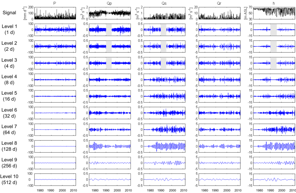
Figure 5: Multiresolution analysis of daily hydrogeological time series using Daubechies 20 wavelets; different components of the decomposition correspond from top to bottom to short-scale to long-time scale processes, with level j corresponding to time scales at 2^{j-1} ; grey rectangles indicate a lack of data for the first levels 1 to 3 (1 to 4-day resolution) during a period of weekly raw data.
