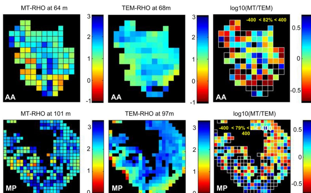
Figure 7 : MT versus TEM resistivity for superficial layers. Above are represented the data of the Anses d'Arlet (AA) geothermal province and below from the Montagne Pelée (MP) geothermal province. Left plots display resistivity from the 3-D MT models for both sector at the indicated depth. Center plots display resistivity of the TEM data (see text for details). Right plots show variation between the two models (log scale).
