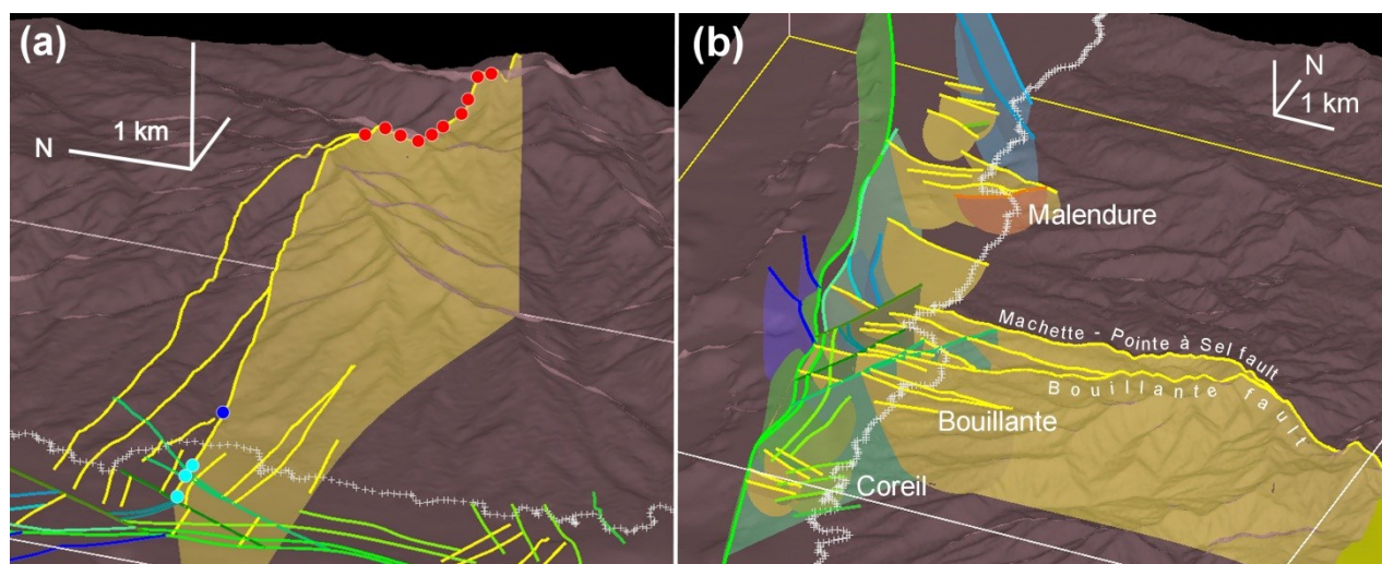
Figure 4: Two views of the fault model achieved for the Bouillante geothermal province (see Fig. 3a for location).
